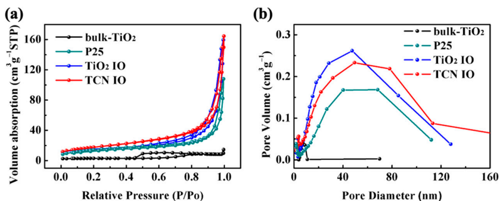
Figure 2. Nitrogen adsorption-desorption isotherms (a) and the corresponding pore size distribution curves (b) of bulk-TiO 2 , TiO 2 IO, TCN IO, P25 sample, respectively.
