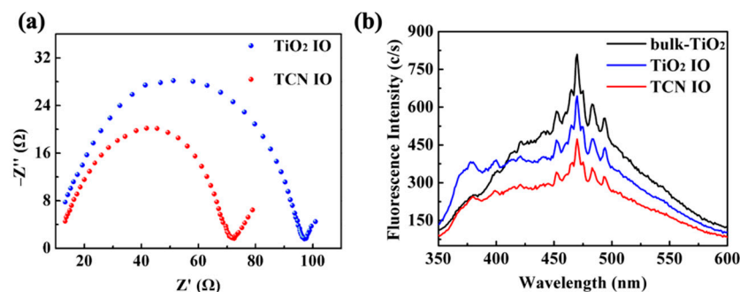
Figure 5. (a) Comparison of the electrochemical impedance spectroscopy (EIS) Nyquist plots for TiO 2 IO and TCN IO, (b) PL spectra of the photocatalysts ( \lambda_{\text{ex}} = 360 \text{ nm} ).
