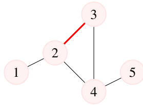
FIG. 1. Computation of the number \alpha_{kl} in an example. The minimal path joining 1 and 2 is P_{12} = 1-2 , P_{13} = 1-2-3 , P_{14} = 1-2-4 , P_{15} = 1-2-4-5 , P_{23} = 2-3 , P_{24} = 2-4 , P_{25} = 2-4-5 , P_{34} = 3-4 , P_{35} = 3-4-5 , P_{45} = 4-5 . It follows that \alpha_{23} = P_{13} + P_{23} = 2 + 1 = 3 .
