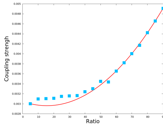
FIG. 9. Fully connected network. Evolution of the coupling strength value g_{20} needed for synchronization with respect to the ratio between random uniform IC and space homogeneous IC in the fully connected network. The blue points represent the values obtained numerically, the red curve represents the function g_n(p) = 352 \times 10^{-9} p^2 - 11 \times 10^{-6} p + 0.00305 .
