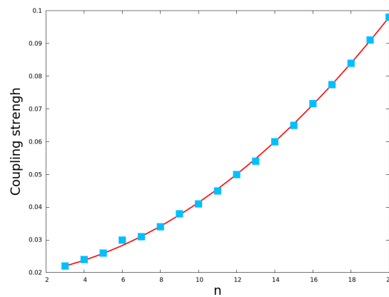
FIG. 10. Unidirectionally ring network. Case c(x) = 0 with spiral and homogeneous IC. Evolution of the coupling strength value g_n needed for synchronization with respect to the number of nodes, n in the graph of the unidirectionally ring network (3.4) with c(x) = 0 , when n varies from 3 to 20. For IC, we choose approximately 50% of spirals and 50% of homogeneous. The blue points represent the values obtained numerically, the red curve represents the function g_n = 0.000169935n^2 + 0.000562092n + 0.0187843 .
