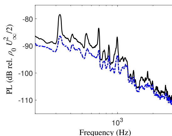
Figure 2. Base wall pressure level (PL) spectra measured at 9.8 \text{ cm} from the upstream edge of a transitional cavity with plain (solid black) or microperforated (dash-dotted blue) floor.
