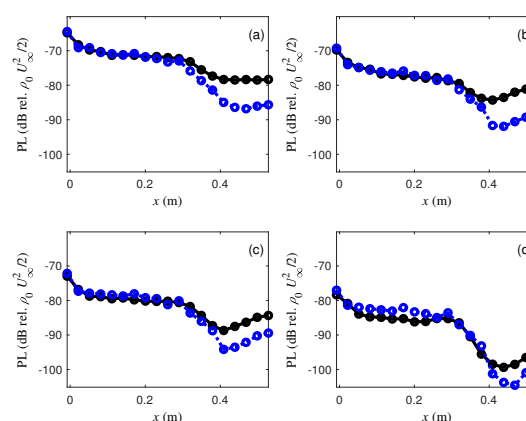
Figure 3. Spatial distribution of the pressure levels (PL) measured along 19 observation points over the base wall of a transitional cavity whose floor was either plain (solid black) or microperforated (dashed blue) at the frequencies (a) 324 Hz, (b) 690 Hz, (c) 990 Hz and (d) 1800 Hz.
