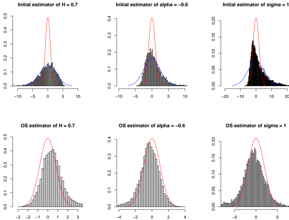
FIGURE 4. Statistical error of the estimators multiplied by \sqrt{n} speed, where \vartheta = (0.7, -0.6, 1) . The first line corresponds to the initial estimator and the second line to the one-step estimator. The blue curves correspond to the density of the centred normal distribution where the theoretical variance is approximated by the empirical variance. The curves in red correspond to the limit law of the one-step estimator.
