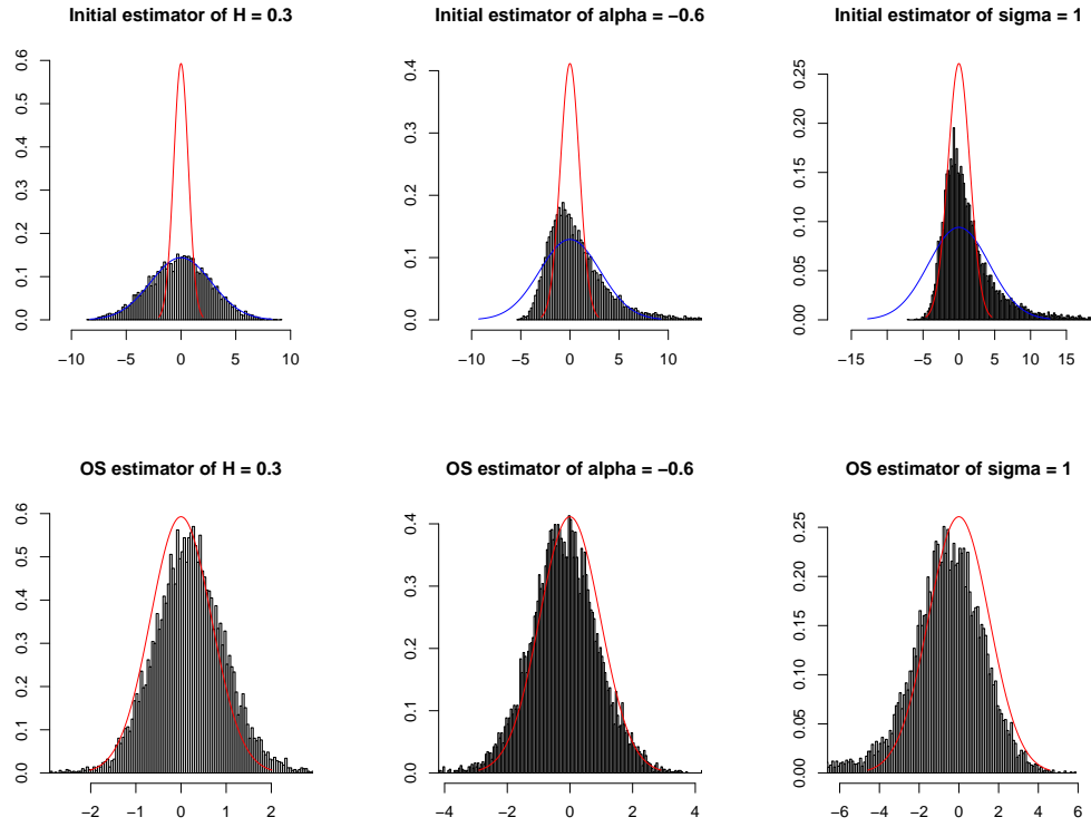
FIGURE 3. Statistical error of the estimators multiplied by \sqrt{n} speed, where \vartheta = (0.3, -0.6, 1) . The first line corresponds to the initial estimator and the second line to the one-step estimator. The blue curves correspond to the density of the centred normal distribution where the theoretical variance is approximated by the empirical variance. The curves in red correspond to the limit law of the one-step estimator.
