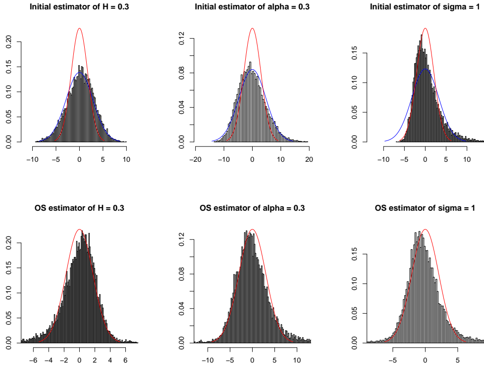
FIGURE 1. Statistical error of the estimators multiplied by \sqrt{n} speed, where \vartheta = (0.3, 0.3, 1) . The first line corresponds to the initial estimator and the second line to the one-step estimator. The blue curves correspond to the density of the centred normal distribution where the theoretical variance is approximated by the empirical variance. The curves in red correspond to the limit law of the one-step estimator.
