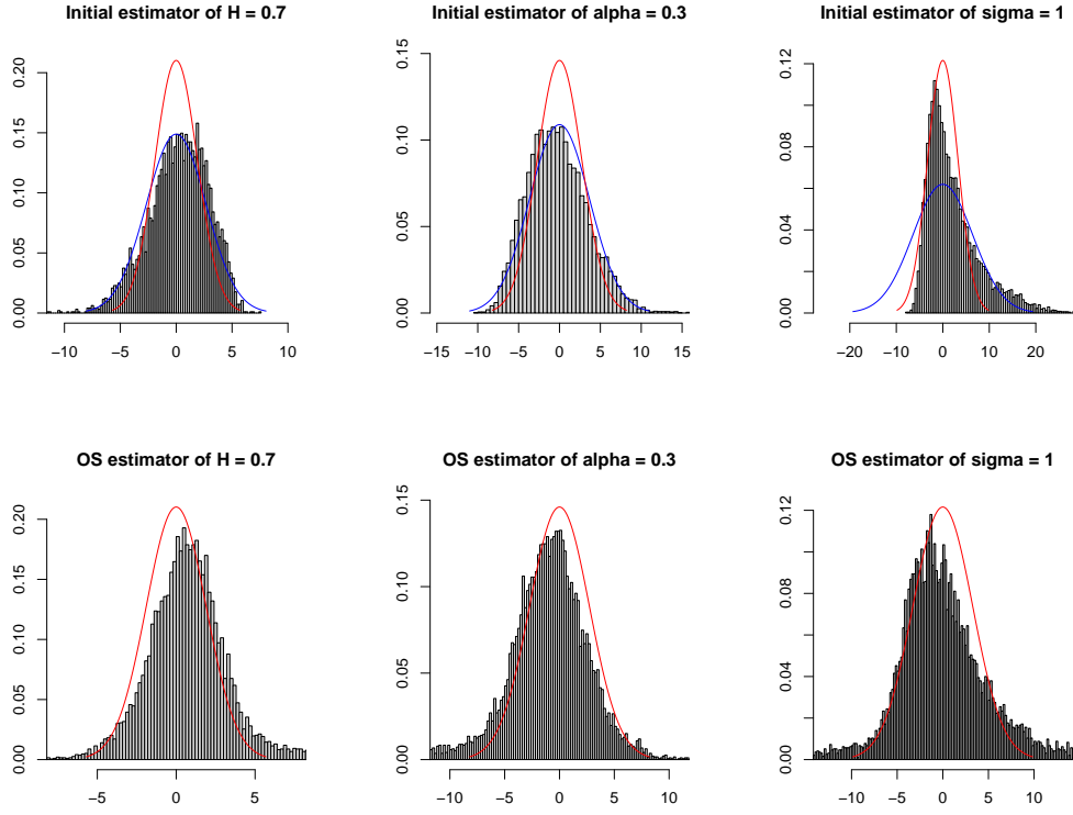
FIGURE 2. Statistical error of the estimators multiplied by \sqrt{n} speed, where \vartheta = (0.7, 0.3, 1) . The first line corresponds to the initial estimator and the second line to the one-step estimator. The blue curves correspond to the density of the centred normal distribution where the theoretical variance is approximated by the empirical variance. The curves in red correspond to the limit law of the one-step estimator.
