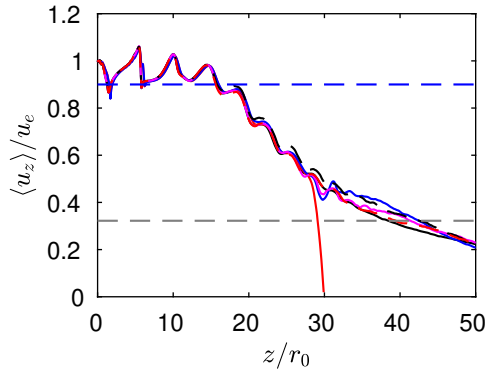
Figure 4. Variations of the mean axial centerline velocity \langle u_z \rangle / u_e for — M31, — M31h0, — M31h13, — M31h2, - - - M31h3 and - - - M31h4; - - - 0.9u_j and - - - c_e .
