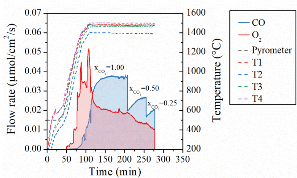
Figure 6: Transient evolution of O 2 and CO production rates along with reactor temperatures, when the inlet CO 2 mole fraction decreases from 1.00 to 0.25 (at 1500°C with Q_{ox, tot}=0.4 L/min).
