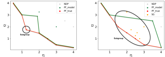
Figure 2: Low entropy (left) and large (right) subgroups.
