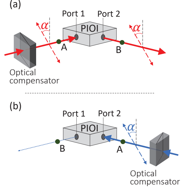
FIG. 5. (Color online) Scheme for investigation of the PIOI in forward (a) and backward (b) directions. In both cases power detection occurs at points A and B, before the entrance port and after the exit port, respectively. The optical compensator allows to prepare any input polarization state (here linearly polarized light under an angle \alpha is shown). The PIOI is the ring arrangement in Fig. 3.
