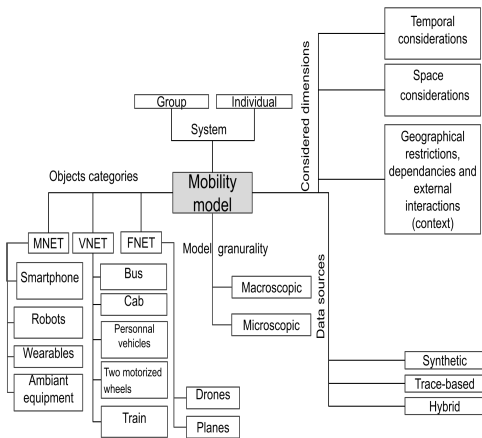
Fig. 1. Mobility models characteristics taxonomy
