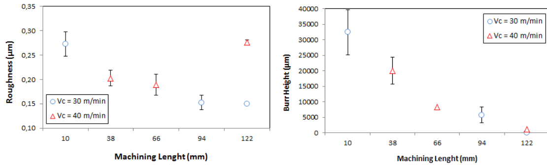
(a) Effect of machining length on surface roughness.
