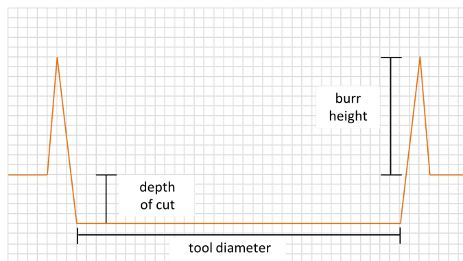
Figure 2. Burr height scheme - front view of the channels
