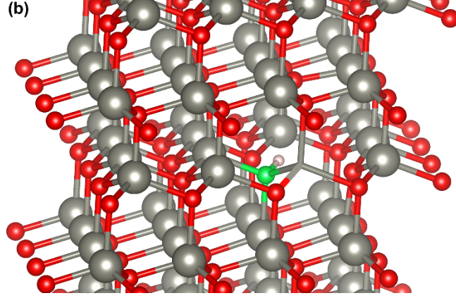
FIG. 6. Structural models for the most stable atomic configuration of the ( V_{Zn} - N_O - H ) defect complex. In (a), the axial ( V_{Zn} - N_O - H ) defect complex is represented. In (b), the basal ( V_{Zn} - N_O - H ) defect complex is represented. The axial configuration is found to be energetically favorable by 0.04 eV with respect to the basal one. Large grey balls, small red balls, small green balls, and small pink balls denote zinc, oxygen, nitrogen, and hydrogen atoms, respectively. The zinc atom in front of the V_{Zn} was taken out for the sake of clarity and only its bonds with the neighboring oxygen atoms are represented.
