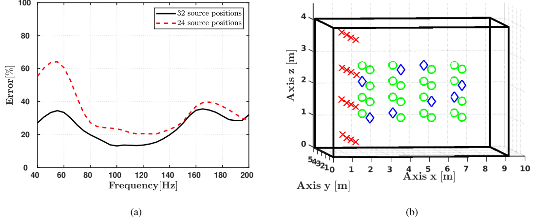
Figure 2: (a) Relative error between direct simulation and estimation of the scattered field, averaged over 16 microphone positions, for 24 and 32 reference source positions. (b) Microphone positions (x); 24 first source positions (o), 8 additional source positions (diamond).
