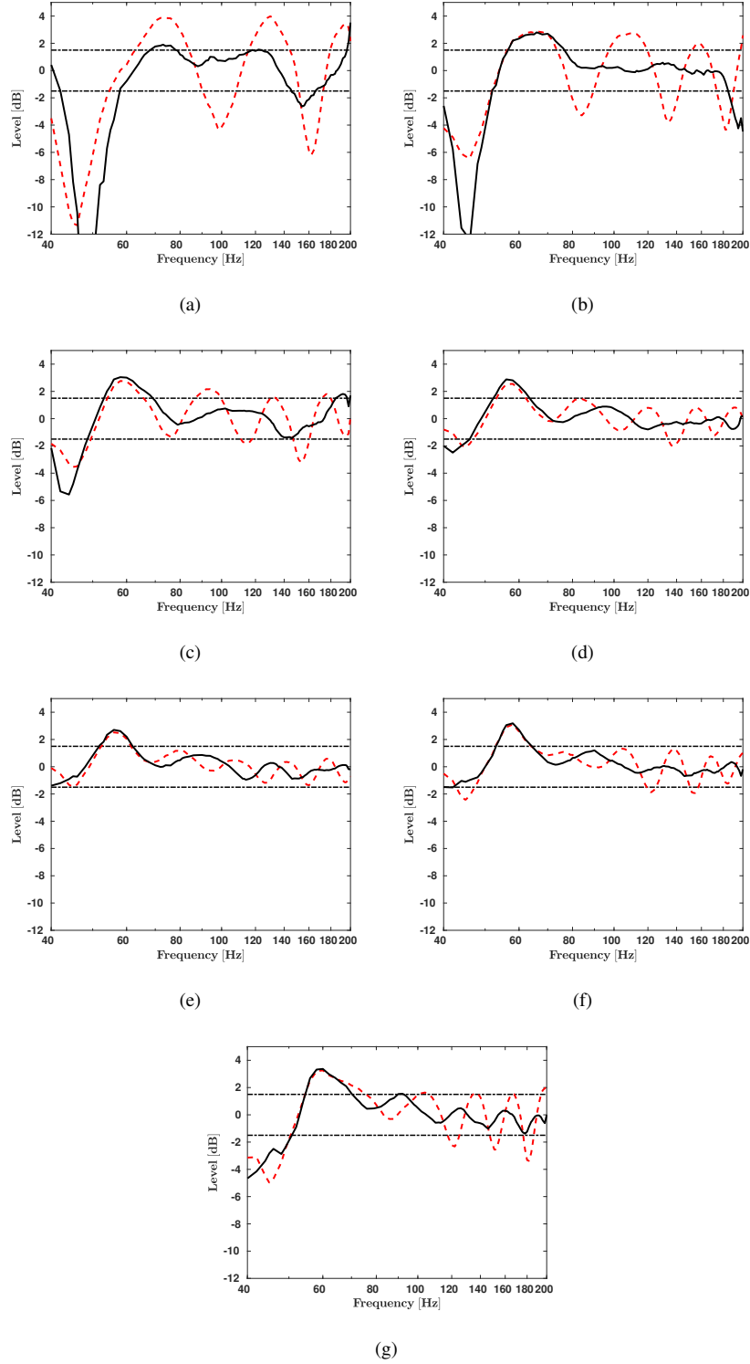
Figure 9: Control on P_\Gamma observed on Q_{\text{Line}} . Control off (—), Control on (—). (a) Q_1 , (b) Q_2 , (c) Q_3 , (d) Q_4 , (e) Q_5 , (f) Q_6 , (g) Q_7 .
