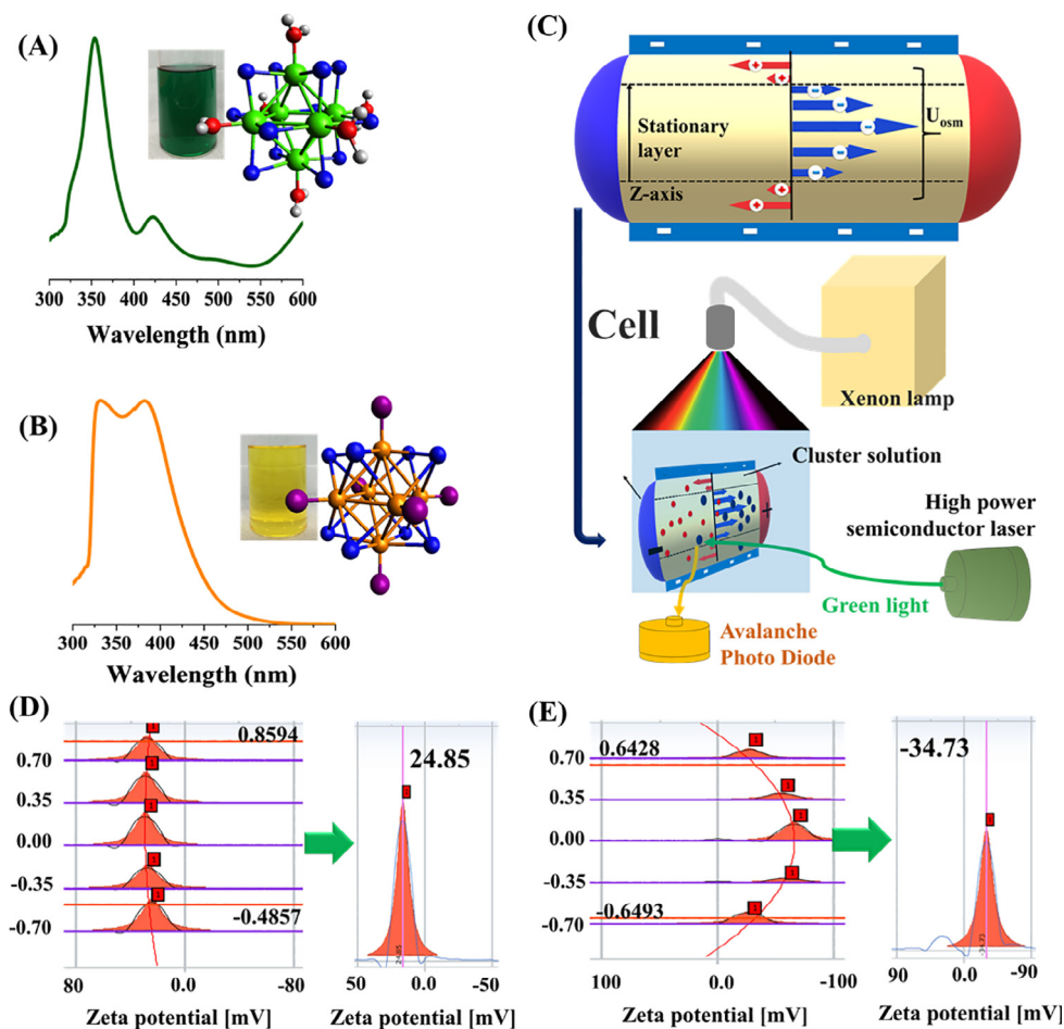
Fig. 1. Optical absorption, MC scheme of A) TBH in acetone/water and B) CMB in MEK. C) Model of the quartz cell and ZP measurement equipped with light irradiation. The ZP value of D) TBH, and E) CMB.
