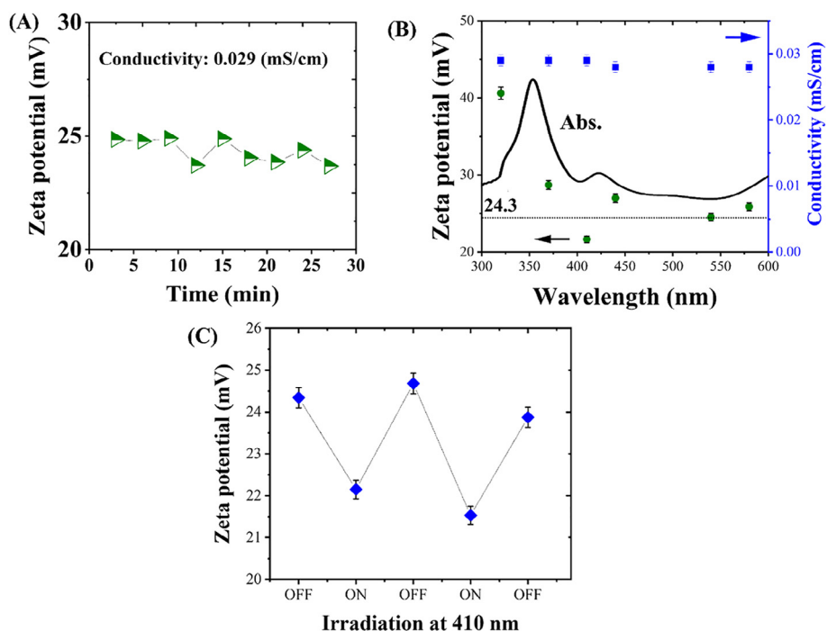
Fig. 3. A) ZP versus time excited at 370 nm and B) the dependence of the ZP and electric conductivity on the irradiation, C) the sensitivity of ZP during light irradiation at 410 nm of the TBH in acetone/water.
