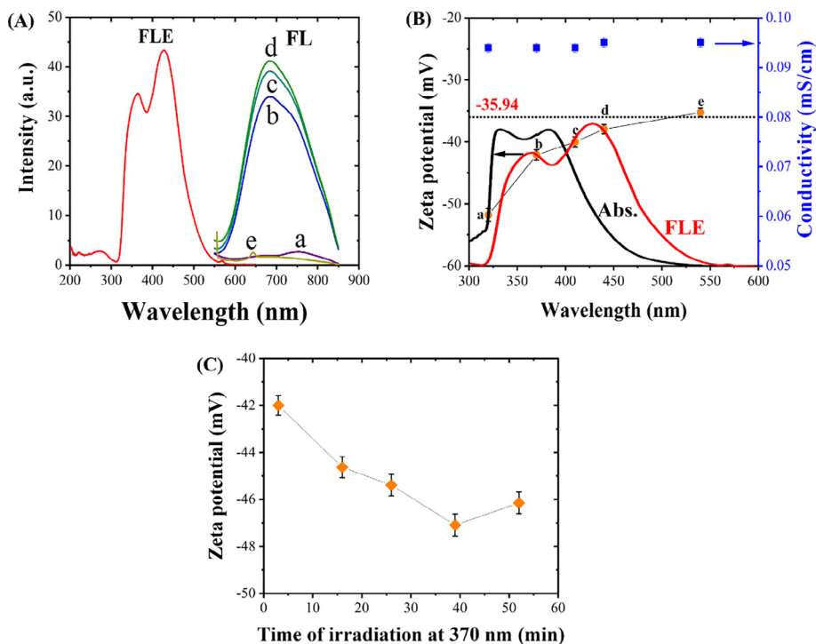
Fig. 2. A) Fluorescence (FL) and fluorescence excitation (FLE) spectra of emission light at 685 nm, B) The dependence of the ZP and electric conductivity of CMB in MEK excited at different wavelengths, and C) ZP versus the irradiation time at 370 nm. The excitation wavelengths of 320, 370, 410, 440, and 540 nm were denoted as the a, b, c, d, and e symbols, respectively.
