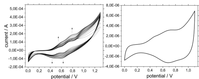
Fig. 8 Multi-scan voltammogram of 2 (left) in DCM with n\text{Bu}_4\text{NPF}_6 as conducting salt and a sweep rate of 200 mV/s on a platinum electrode. After washing the electrode with DCM a voltammogram (right) in a monomer-free DCM solution with n\text{Bu}_4\text{NPF}_6 was conducted.
