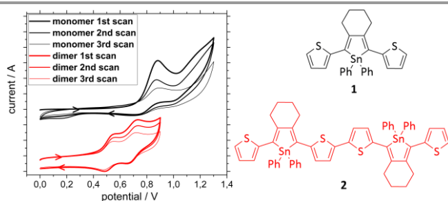
Fig. 6 Cyclic voltammogram of stannole 1 (black) and 2 (red) in DCM with n\text{Bu}_4\text{NPF}_6 as conducting salt using platinum working electrodes.
