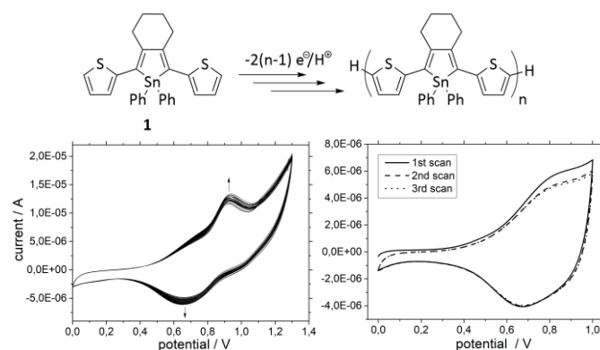
Fig. 7 Multi-scan voltammogram of 1 (left) in DCM/ n -pentane (1/1) with n\text{Bu}_4\text{NPF}_6 as conducting salt and a sweep rate of 200 mV/ s on a platinum electrode. After washing the electrode with DCM, a voltammogram (right) in a monomer-free DCM/ n -pentane (1/1) solution with n\text{Bu}_4\text{NPF}_6 was conducted.
