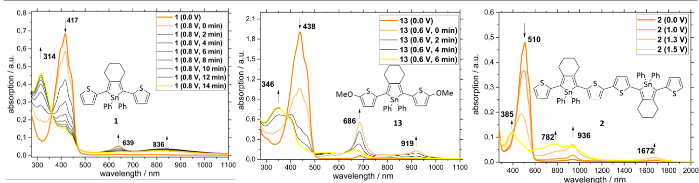
Fig. 9 (Left) Stacked absorption spectra of stannole 1 in DCM with n\text{Bu}_4\text{NPF}_6 as conducting salt upon oxidation starting from 0.80 V and recording a spectrum every 2 min. (Middle) Stacked absorption spectra of 13 in DCM with n\text{Bu}_4\text{NPF}_6 as conducting salt upon oxidation. (Right) Stacked absorption spectra of stannole 2 in DCM with n\text{Bu}_4\text{NPF}_6 as conducting salt upon oxidation. As 2 decomposed immediately upon oxidation, the voltage was increased gradually (every 2 min) to generate dope species. In all cases the concentration was 10^{-4} M.
