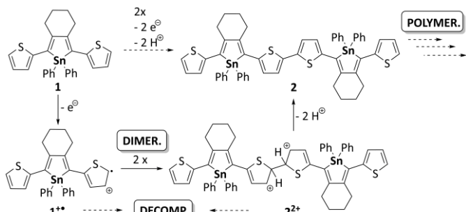
Scheme 2 Proposed mechanism of an oxidative polymerization of thienyl-substituted 1 including the formation of stannole radical cation 1 •+ , dimer dication 2 •• and the dimer 2 . The decomposition of the stannole species could also occur as side-reaction.
