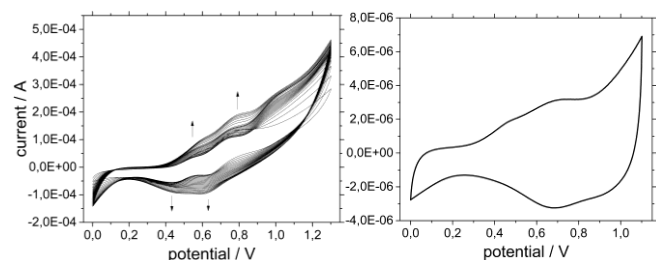
Fig. 8 Multi-scan voltammogram of 2 (left) in DCM with n\text{Bu}_4\text{NPF}_6 as conducting salt and a sweep rate of 200 mV/s on a platinum electrode. After washing the electrode with DCM a voltammogram (right) in a monomer-free DCM solution with n\text{Bu}_4\text{NPF}_6 was conducted.
