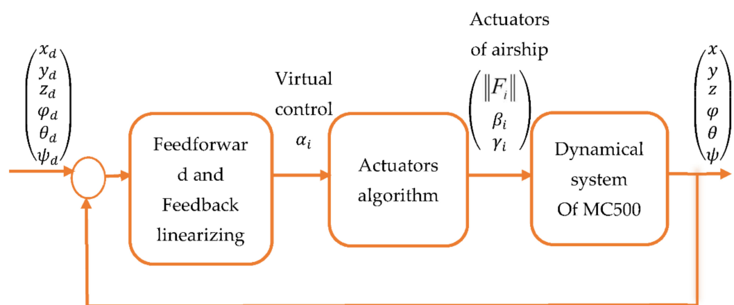
Figure 5. Closed-loop architecture of control.
