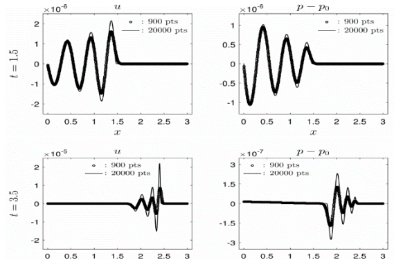
Figure 5. Cont. of Figure 4 with A = 1.0e-6 .
