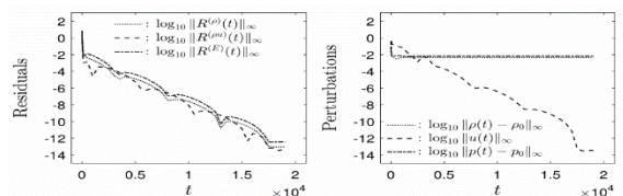
Figure 6. The convergence to the steady state of the numerical solution of perturbation from polytropic equilibrium : A = 1.0e-1 .
