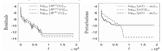
Figure 7. Cont. of Figure 6 with A = 1.0e-6 .
