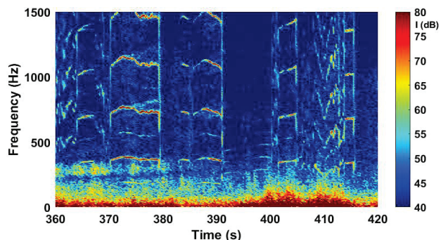
Figure 16. Spectrogram of a Parrot Disco (outdoor)
