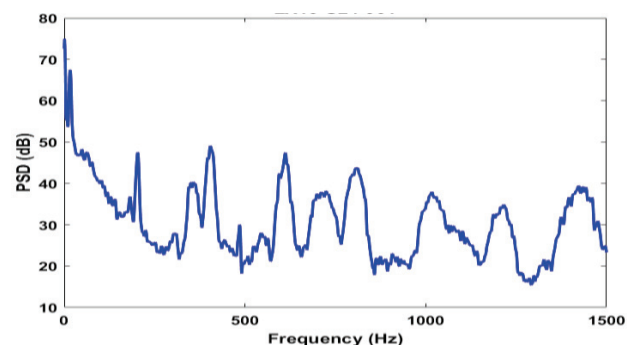
Figure 15. Spectrum of a DJI Phantom 3 (outdoor)
