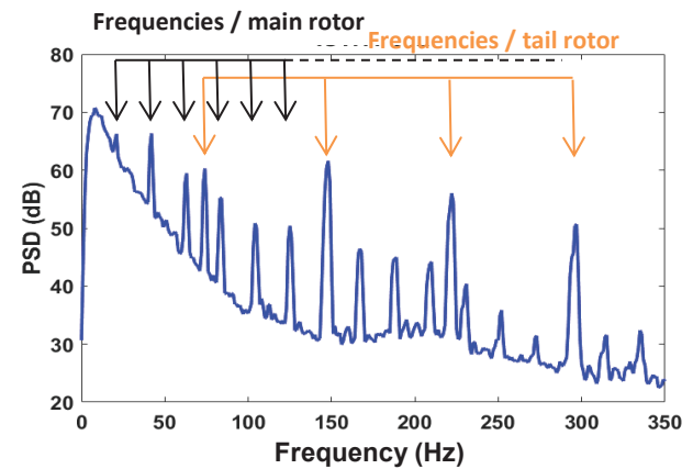
Figure 4. Example of spectrum of a helicopter noise
