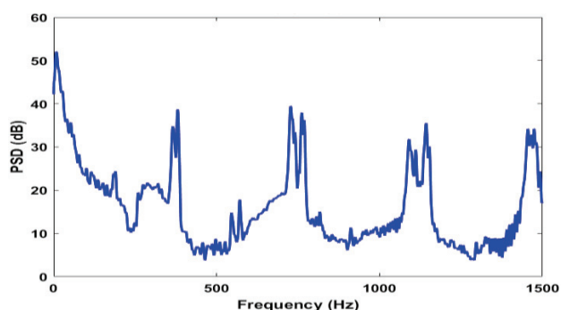
Figure 17. Spectrum of a Parrot Disco (outdoor)
