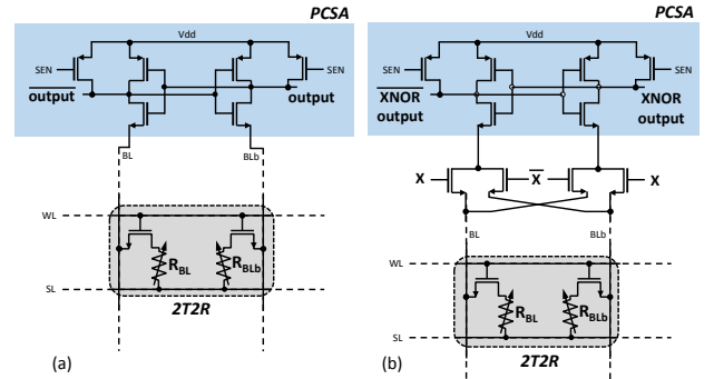
Fig. 3. (a) Schematic of the sense amplifier used to extract the binary weight from a 2T2R synapse. (b) Version augmented with an XNOR feature.
