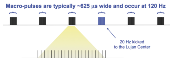
Figure 3: Shown here is an illustration of the WNR beam structure. Micropulses of protons approximately 150 ps wide are separated by approximately 1.8 \mu\text{s} from neighboring micropulses, and are bunched into macropulses. Macropulses are approximately 347 micropulses long, and are separated from neighboring macropulses by approximately 8.3 ms, with the exception of times when a macropulse is alternatively sent to the LANSCE Lujan center. This figure is a reproduction of Fig. 1 of Ref. (24).
