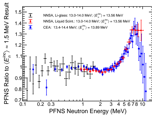
Figure 16: (color online) Shown here is a comparison of CEA (full, blue squares) and NNSA (Li-glass data shown as full, black diamonds and liquid scintillator data shown as full, red circles) PFNS results at at \langle E_n^{inc} \rangle \approx 13.5 \text{ MeV} shown as a ratio to the result at \langle E_n^{inc} \rangle \approx 1.5 \text{ MeV} for each measurement.
