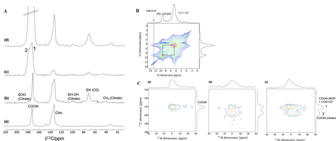
Figure 6. NMR spectra of MIL-100(Al), CD-CO@nanoMIL-100(Al), CD- ^{13}\text{C} @nanoMIL-100(Al), and DOX loaded CD- ^{13}\text{C} @nanoMIL-100(Al). (A). ^{13}\text{C} CPMAS NMR spectra of (a) MIL-100(Al), (b) CD-CO@nanoMIL-100(Al), (c) CD- ^{13}\text{C} @nanoMIL-100(Al), and (d) DOX loaded CD- ^{13}\text{C} @nanoMIL-100(Al). In (d), the small unlabeled peaks correspond to the DOX molecules. The intense ^{13}\text{C} resonances is truncated for sake of clarity. In (c), 1 and 2 show the two labeled carboxylic resonances. Line 2 corresponds to the ^{13}\text{C} carboxylic atoms of the CO linked to the surface aluminum sites of the MOF. Line 1 is a superimposition of COOAl carboxylic of the trimesate BTC linker and the ^{13}\text{C} COO-CD of the polymer coating. (B). ^1\text{H} - ^1\text{H} 2D MAS NMR spectrum of DOX loaded CD- ^{13}\text{C} @nanoMIL-100(Al) dried. (C). 2D ^{13}\text{C} - ^{27}\text{Al} D-HMQC 2D of (a) nanoMIL-100(Al), (b) CD- ^{13}\text{C} @nanoMIL-100(Al) and (c) DOX loaded CD- ^{13}\text{C} @nanoMIL-100(Al).
