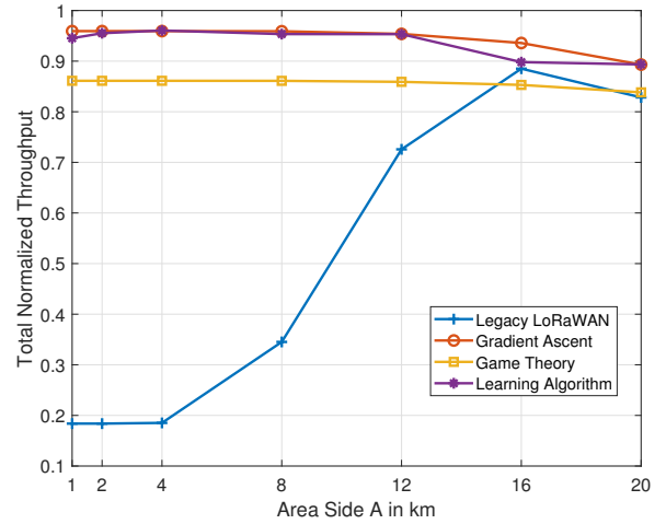
Fig. 14. Impact of the area size on the total normalized throughput
