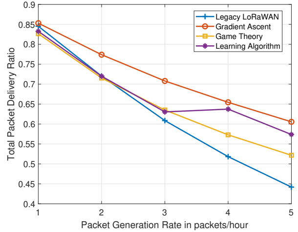
Fig. 11. Impact of packet generation rate on total packet delivery ratio
