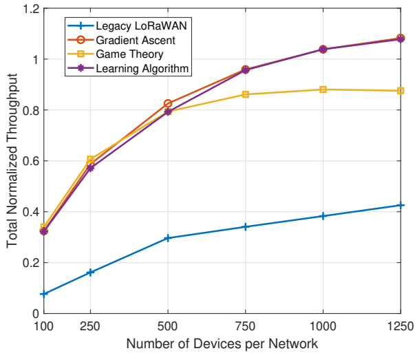
Fig. 12. Impact of the number of devices on the total normalized throughput
