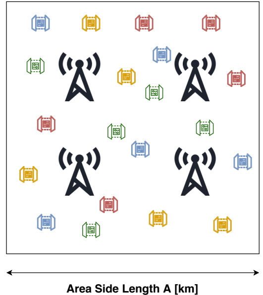
Fig. 1. A 4 gateway multi-operator LoRaWAN deployment
