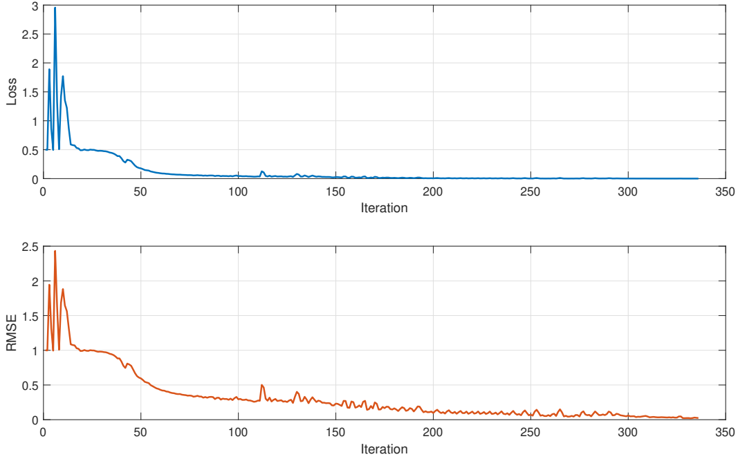
Fig. 6. Training progress for success rate prediction
