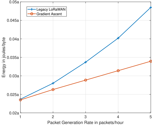
Fig. 18. Energy consumed per delivered byte as a function of the packet generation rate
