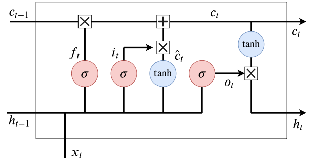
Fig. 4. An LSTM unit
