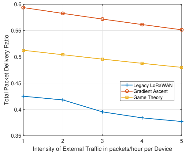
Fig. 17. Impact of external traffic from non-cooperative source on the total packet delivery ratio
