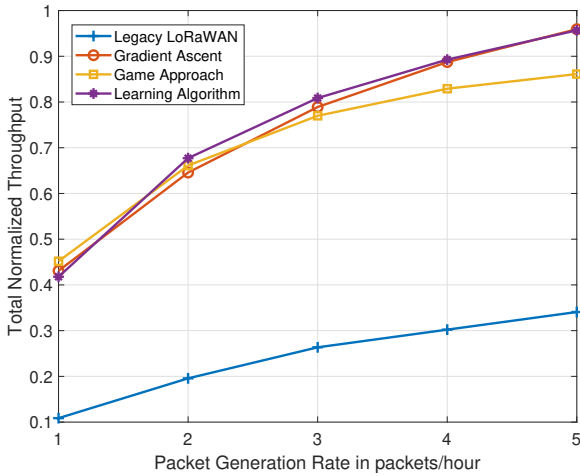
Fig. 10. Impact of packet generation rate on total normalized throughput
