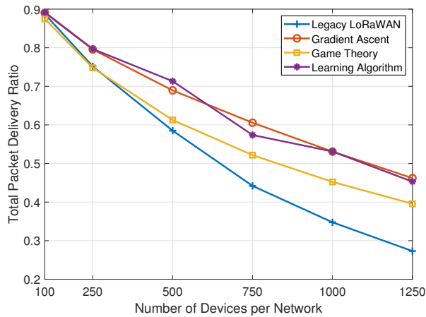
Fig. 13. Impact of the number of devices on the total packet delivery ratio
