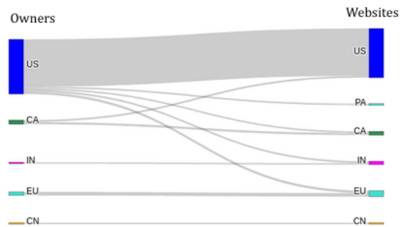
Fig. 8. Cookie respawning with browser fingerprinting is geologically distributed. Corresponding countries of owners (left) and websites including respawning (right) of respawnd cookies. We present the top 10 (owner,website) geolocation. "EU" label represents the 27 member states of the EU.
