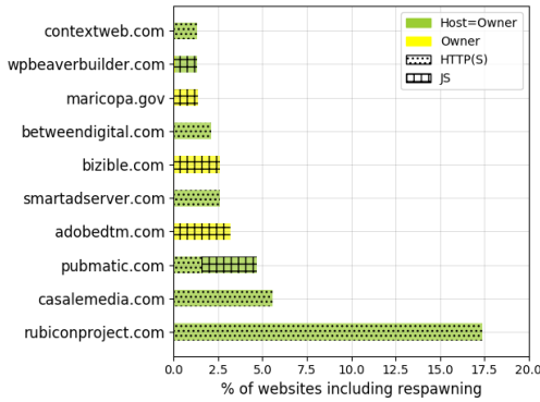
Fig. 5. The top 10 respawnd cookies owners. The bar is green when the domain is both host and owner, and yellow when the domain only appears as owner. For each domain, we show when cookies are set via an HTTP(S) header and when they are set via JavaScript. When considering cookie owners, new domains are identified such as adobedtm.com.
