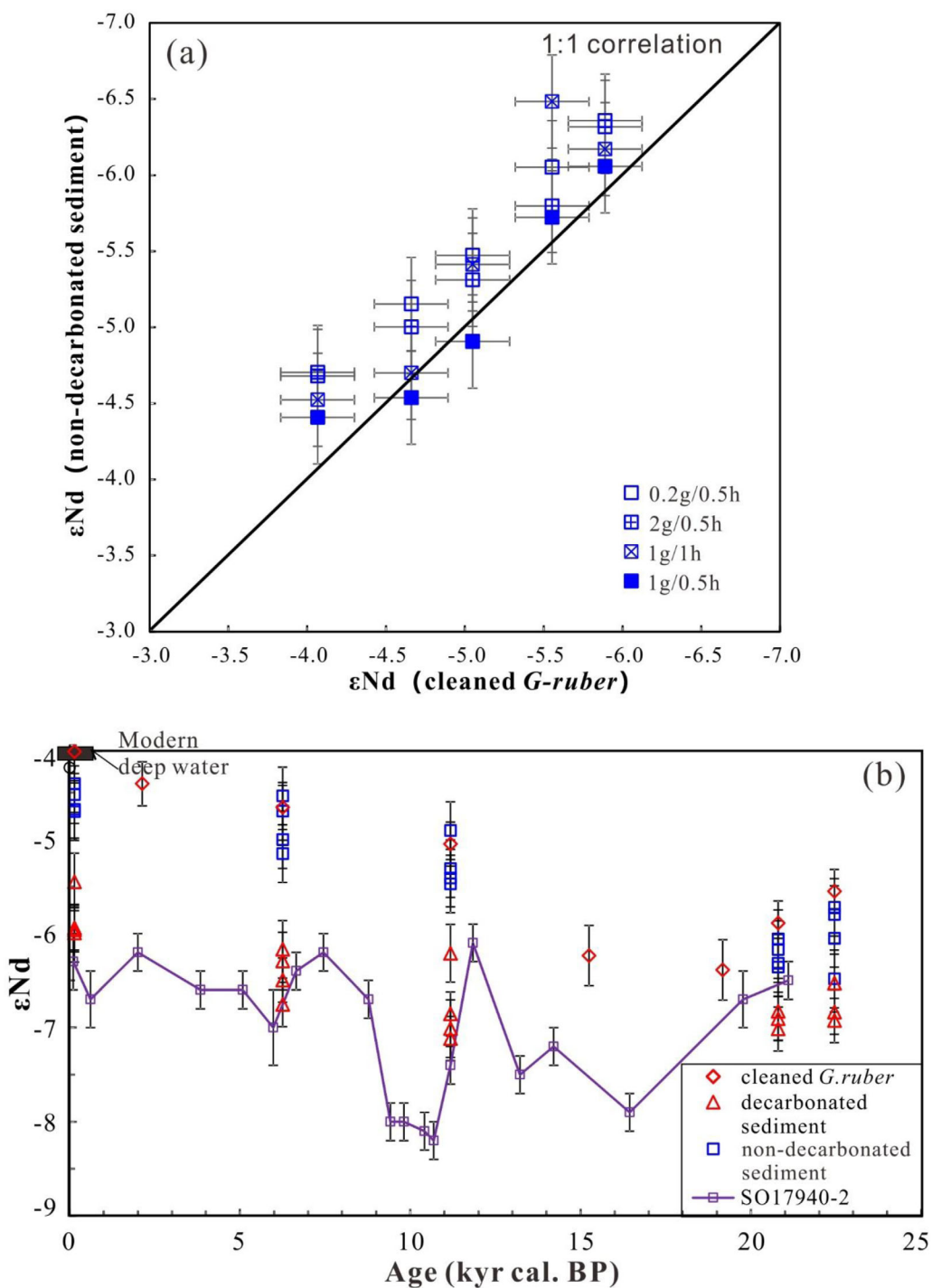
Figure 6. (a) Crossplot of \epsilon\text{Nd} values of non-decarbonated sediment leachates and \epsilon\text{Nd} values obtained from cleaned planktonic foraminifera G. ruber . (b) \epsilon\text{Nd} values obtained from acid-reductive HH leachates of bulk non-decarbonated and decarbonated sediments of core MD05-2904. \epsilon\text{Nd} values have been obtained by using HH leaching of 0.2, 1, and 2 g samples of sediments leached for 0.5, 1, 2, and 3 h. \epsilon\text{Nd} obtained on seawater samples close to the studied site [Wu et al. , in press] as well on cleaned planktonic foraminifera G. ruber of core MD05-2904 are also reported. \epsilon\text{Nd} from acid-reductive HH leachates of bulk decarbonated sediments of the core SO17940-2 [Huang et al. , 2013] are also reported for comparison.
