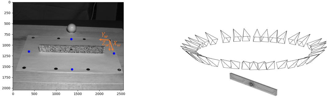
(a) Example of an input image used for the shape and albedo scan. Superimposed blue dots stand for the light calibration points. The world reference frame is shown in orange. Both were not present in the original picture.
