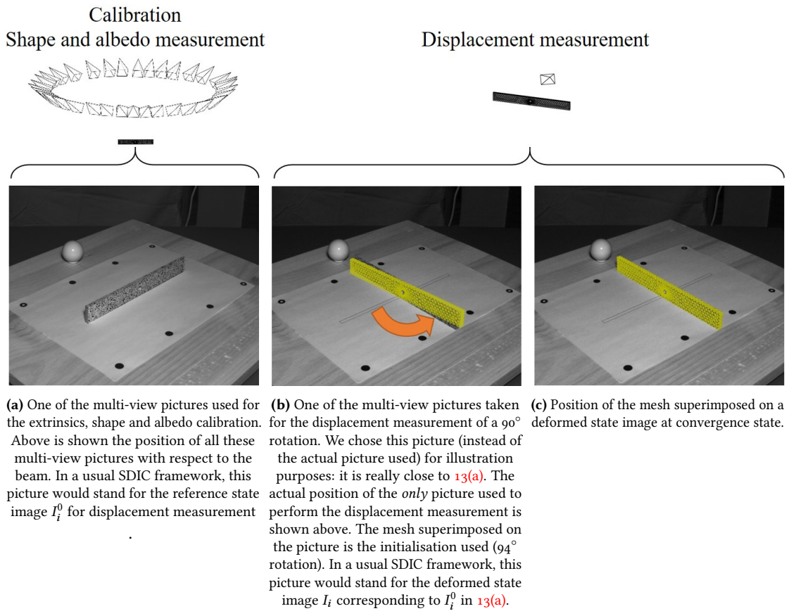
Figure 13: This Figure allows to explain the approach followed and how difficult it would be to measure this 90^\circ rotation in a usual SDIC framework. As the displacement measurement step in classic SDIC would be based on the comparison between reference state images I_i^0 13(a) and deformed state ones I_i 13(b) that observe different faces of the specimen.
