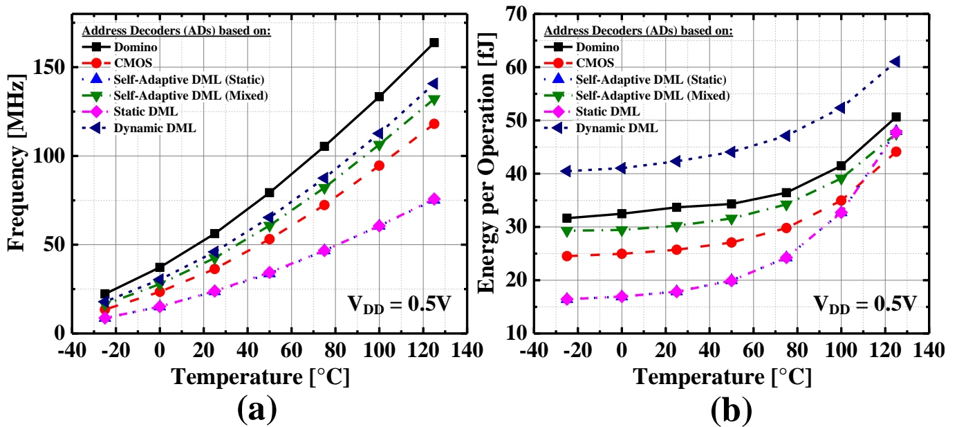
Figure 7. Address Decoder temperature variation analysis from -25\text{ }^{\circ}\text{C} to 125\text{ }^{\circ}\text{C} at 0.5 V for: (a) Frequency. (b) Energy.
