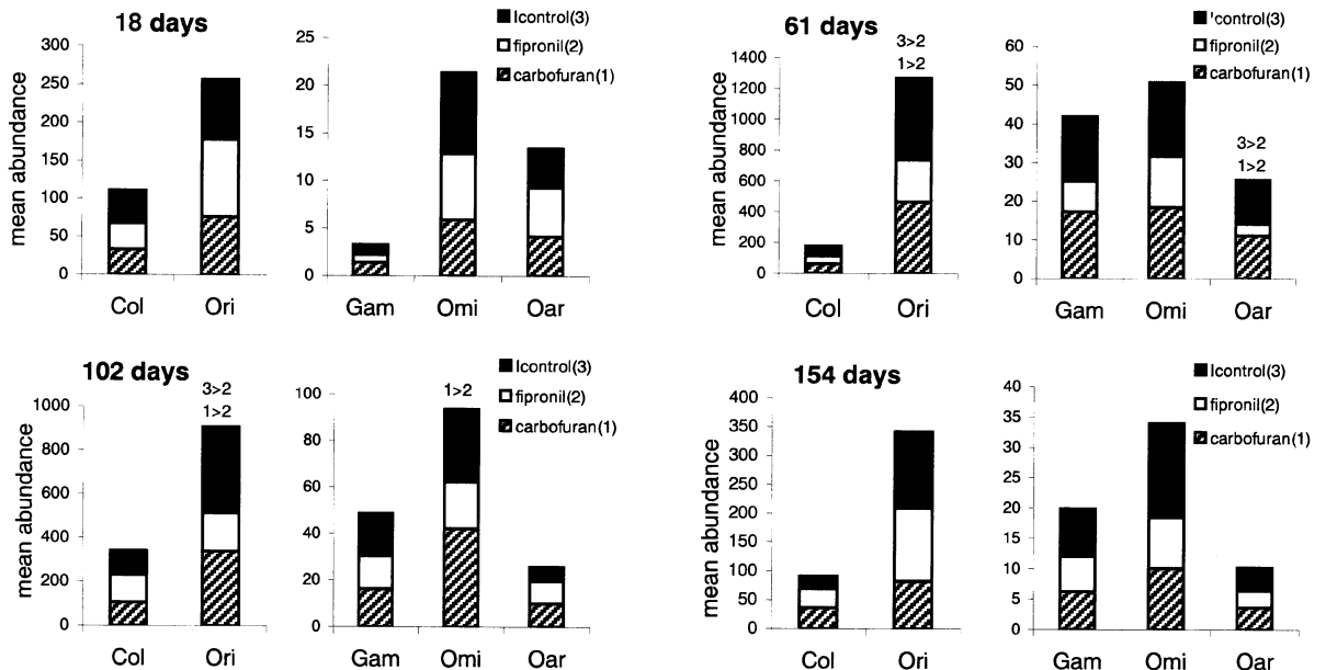
Fig. 2. Mean abundance of microarthropods (number of individuals/litterbag) in the insecticide section for each treatment (fipronil, carbofuran, I-control) and each sampling date (18, 61, 102, 154 days). Col, Collembola; Ori, Oribatida; Gam, Gamasida; Omi, other mites; Oar, other arthropods. Significant differences between treatments (ANOVA, P < 0.05 ) are noted on the relevant histograms.
