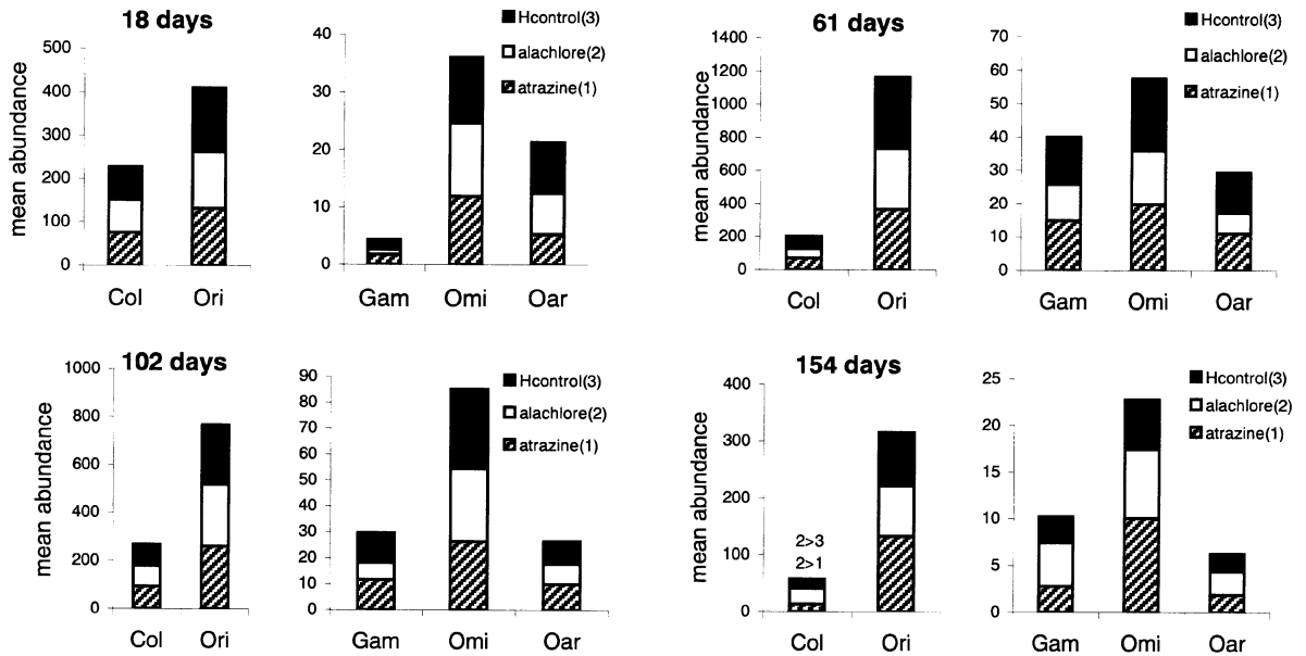
Fig. 1. Mean abundance of microarthropods (number of individuals/litterbag) in the herbicide section for each treatment (atrazine, alachlore, H-control) and each sampling date (18, 61, 102, 154 days). Col, Collembola; Ori, Oribatida; Gam, Gamasida; Omi, other mites; Oar, other arthropods. Significant differences between treatments (ANOVA, P < 0.05 ) are noted on the concerned histograms.
