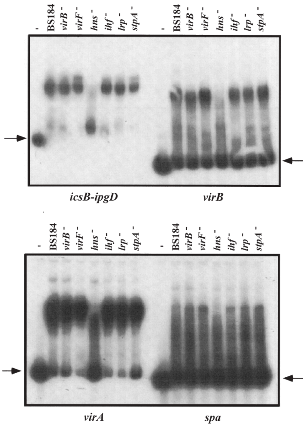
Fig. 3. Retardation of fragments of the icsB-ipgD intergenic region and virB (upper panel), and virA and spa (lower panel) promoter regions with crude cell extracts from BS184 and its virB , virF , hns , ihf , lrp and stpA mutant derivatives (Table 1). Complexes were resolved through a 6% polyacrylamide gel in 0.5X TBE at 4°C. Arrows correspond to unbound DNA.
