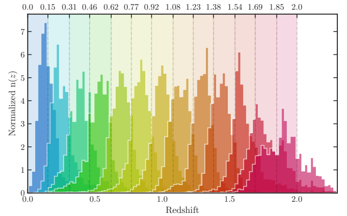
Fig. 8. Redshift distributions ( z_{mc} ) of the 13 bins with an equal width for the fiducial sample (case 2). The top x -axis correspond to the values of the redshift limits of the 13 bins with an equal width in redshift. The shaded regions indicate these limits.
