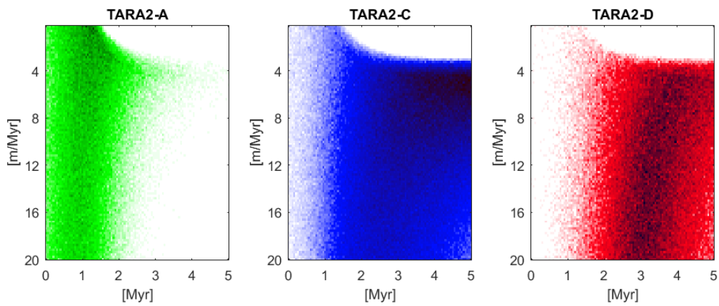
Figure S 14. Same as Figure S 5 for site TARA2.
