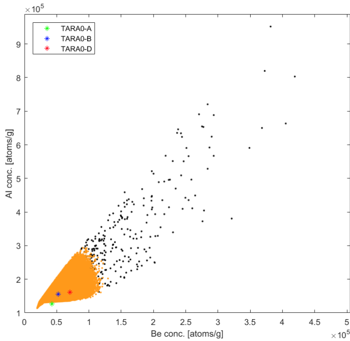
Figure S 9. Same as Figure S3 for site TARA0.
