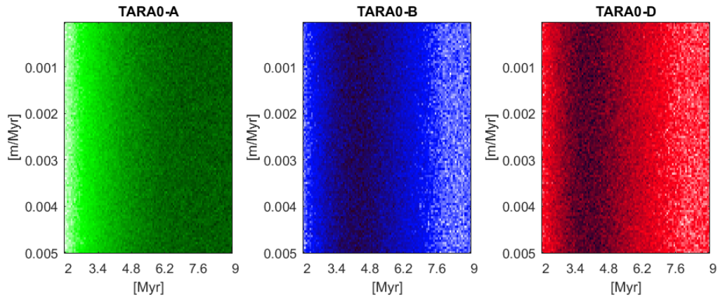
Figure S 11. Same as Figure S 5 for site TARA0.
