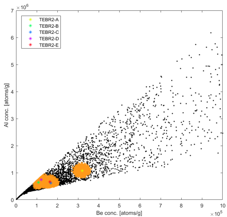
Figure S 6. Same as Figure S3 for site TEBR2.
