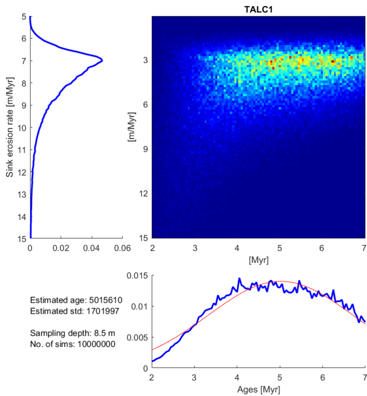
Figure S 16. Same as Figure S 4, for site TALC1; it corresponds to an age of 5,015,610 \pm 1,701,997 a.
