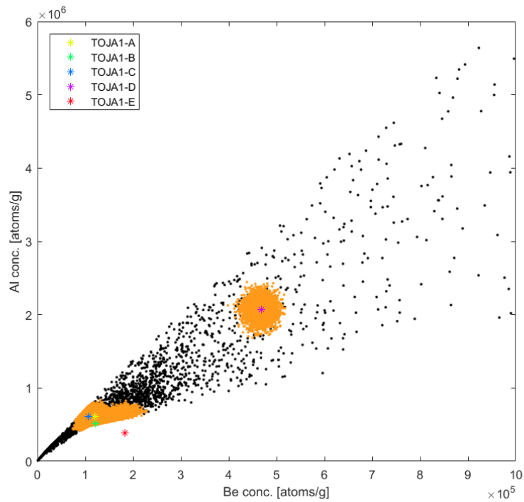
Figure S3. Inventory of 0.1% of the cosmogenic pairs ( ^{26}\text{Al} , ^{10}\text{Be} ) produced by the P-PINI burial-age model (black dots) for site TOJA1. Colored stars show the ( ^{26}\text{Al} , ^{10}\text{Be} ) inventories of the five samples from TOJA1 site. Orange dots show the simulated ( ^{26}\text{Al} , ^{10}\text{Be} ) concentrations accepted by P-PINI; the entire inventory of accepted concentrations is displayed.
