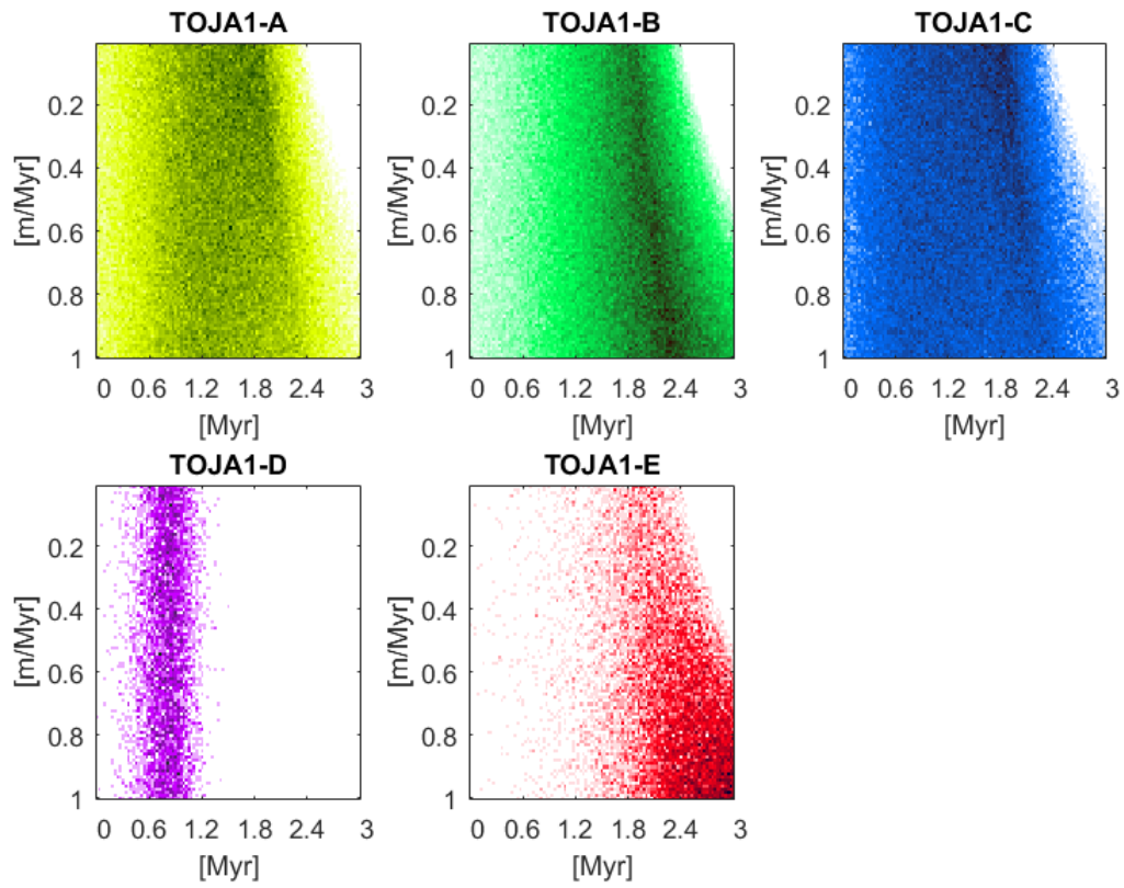
Figure S 5. Erosion rates and burial ages associated with the accepted P-PINI simulations for each one of the five samples from TOJA1 site. Darker colors indicate higher number of accepted simulations. Note that Figure S3 represents the common signal deduced from the five samples taken altogether.
