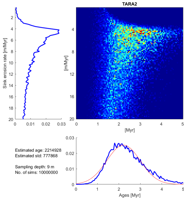
Figure S 13. Same as Figure S 4, for site TARA2; it corresponds to an age of 2,214,928 \pm 777,868 a.
