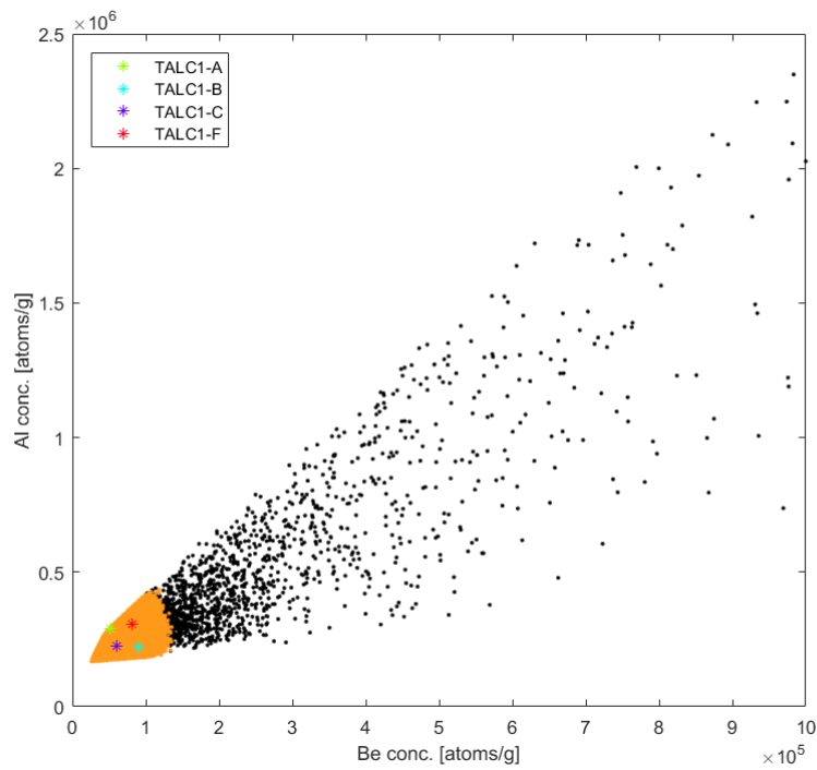
Figure S 15. Same as Figure S3 for site TALC1
