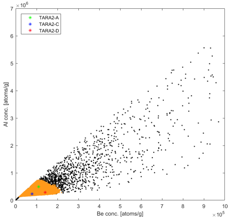
Figure S 12. Same as Figure S3 for site TARA2
