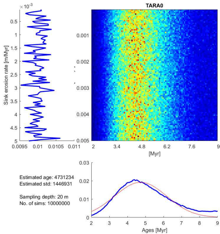
Figure S 10. Same as Figure S 4, for site TARA0; it corresponds to an age of 4,731,234 \pm 1,446,931 a.
