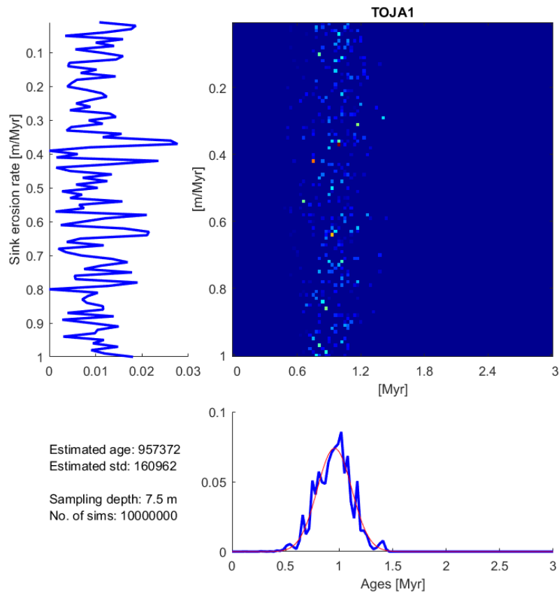
Figure S 4. Center panel: the combined probability density distribution for the burial age and erosion rate of TOJA1 site, obtained by multiplying together the probability distributions associated with each of the five samples from this site. Dark blue denotes zero probability, whereas light-blue and reddish colors denote higher probability. Left panel: the marginal probability distribution for the erosion rate (blue line). From this graph no clear erosion rate for sink (site TOJA1, erosion of the terrace surface) can be deduced. Bottom panel: the marginal probability distribution for the burial age (blue line). The red line denotes the Gaussian fit to the probability distribution for the burial age. The probability distribution corresponds to an age of 957,372 \pm 160,962 a for TOJA1 terrace deposits.
