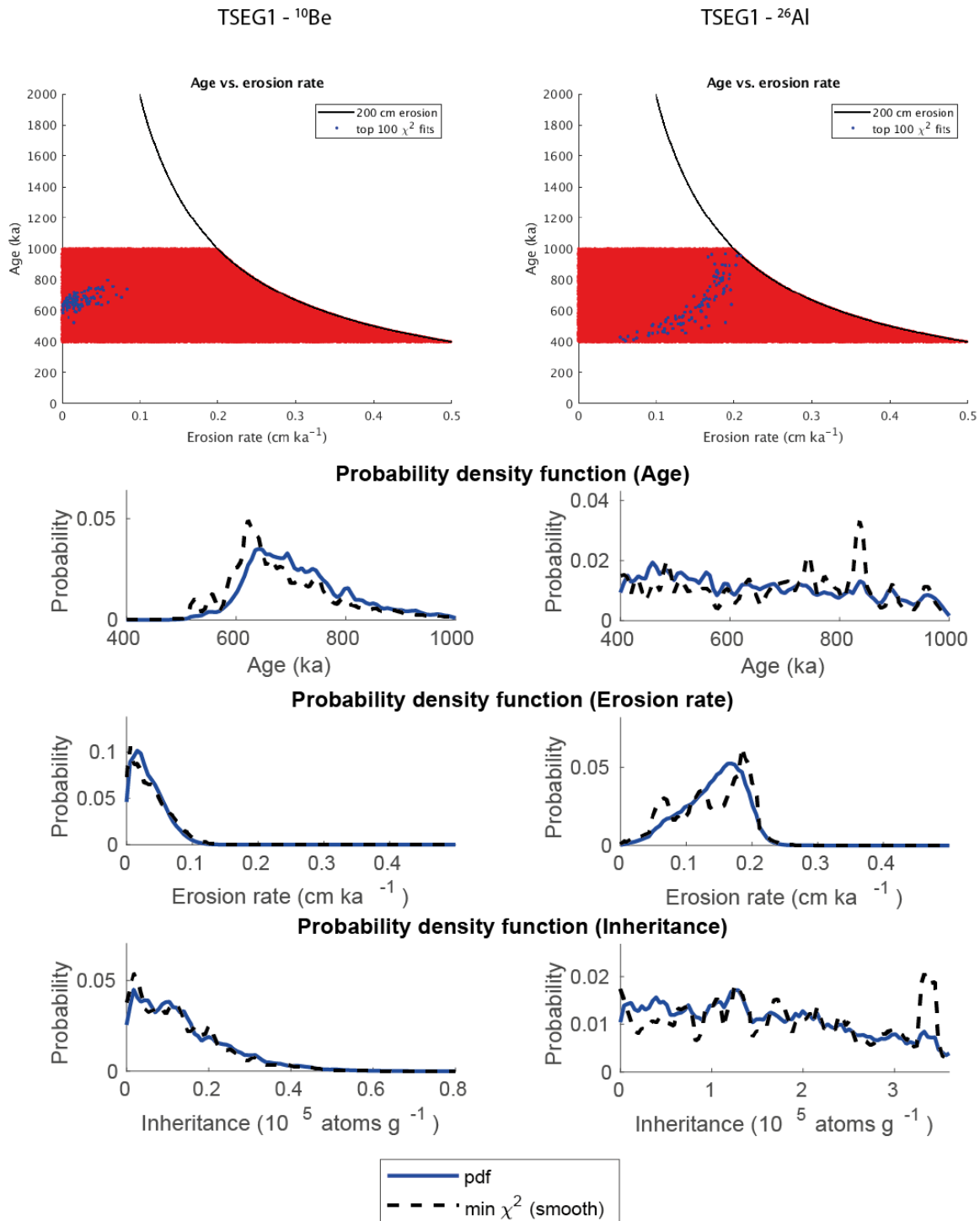
Figure S2. Selected graphical outputs of the Hidy et al. (2010) inversion program (depth profile is in Figure 8 of the main text), for the TSEG 1 profile; for ^{10}\text{Be} and ^{26}\text{Al} data on the left and right respectively. The top graphs show the range of parameters tested (red), in which the 100 most reliable are shown in blue (best \chi^2 ). The corresponding probability density functions are shown in the lower graphs, for age, erosion rate or inheritance.
