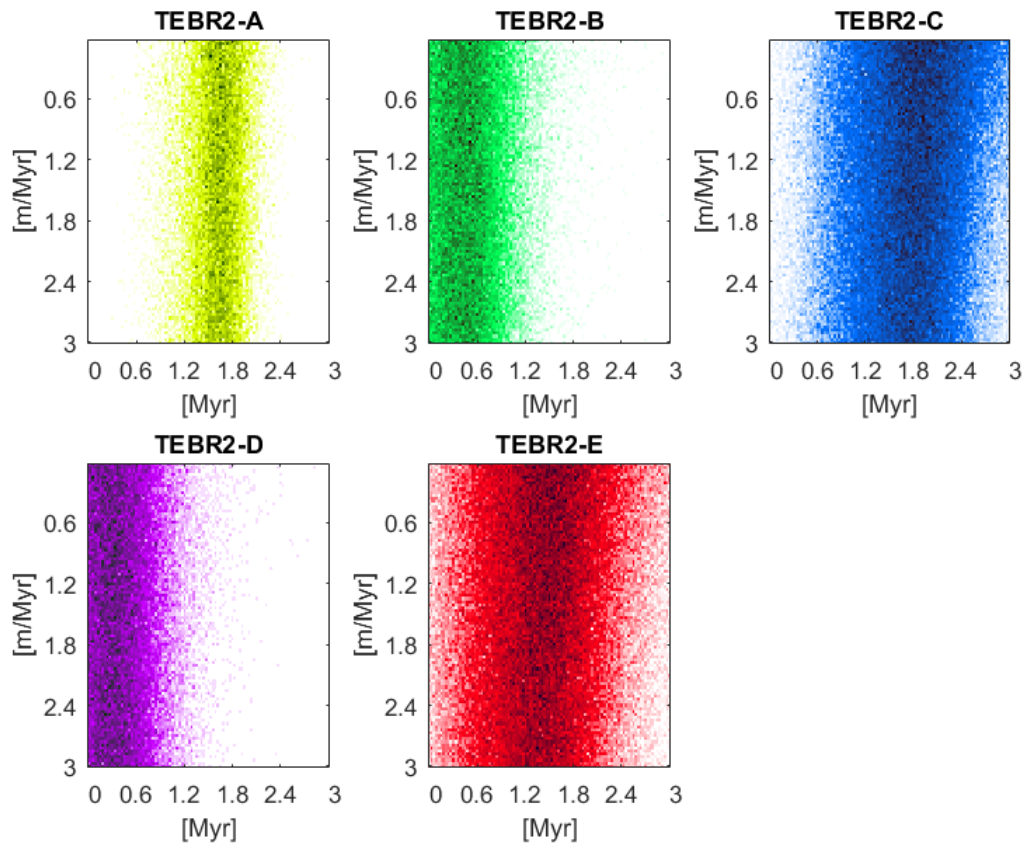
Figure S 8. Same as Figure S 5 for site TEBR2.
