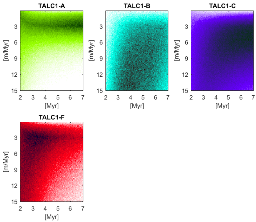
Figure S 17. Same as Figure S 5 for site TALC1.
