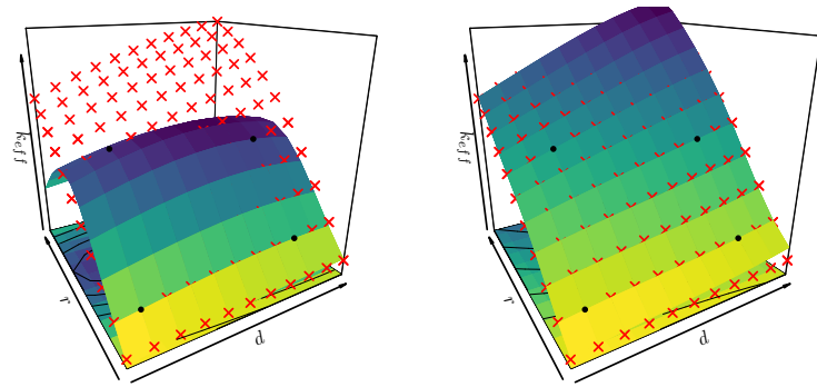
FIGURE 8 – Left : uncertainty reduction of a 2D function, when adding monotonicity and box constraints. Top : prediction surface of a criticality coefficient in nuclear engineering with 4 observations (bullets), without constraints (left) or accounting for monotonicity and positivity (right). Crosses represent test points.
