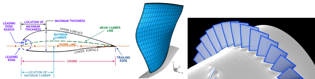
FIGURE 5 – The rotor test case : the blades are described by 4 cross-sections for a total of 20 design parameters. There are uncertainties about the manufacturing (rugosity, tip gap), the inflow properties (pressure, temperature and azimuthal momentum) and operational conditions (flow rate, rotation speed). These 7 uncertain parameters affect 5 constraints about the inlet and outlet relative flow angles, the flow speed reduction, excessive loading and the Mach number of the blade tips. The objective function is the polytropic (compressor) efficiency.
