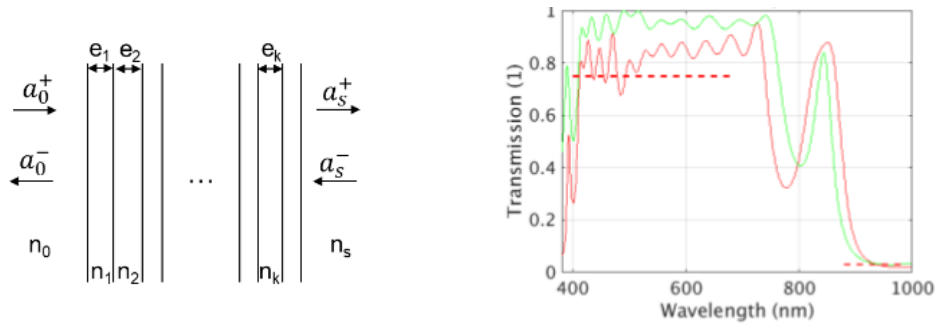
FIGURE 4 – Design of a multilayer filter for light radiations. The design variables are the materials of the layers (labelled 'n'), which are categorical, and the layers' thicknesses (labelled 'e'), which are continuous. The objective function is a distance to a target of the transmission spectrum.
