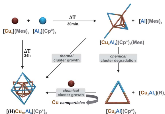
Scheme 2 Synthetic pathways to the new Cu/Al clusters [\text{Cu}_4\text{Al}_4](\text{Cp}^*)_5(\text{Mes}) (1), [\text{Cu}_2\text{Al}](\text{Cp}^*)_3 (2), and the inseparable mixture of [\text{HCu}_7\text{Al}_6](\text{Cp}^*)_6 (3 H ), [\text{Cu}_7\text{Al}_6](\text{Cp}^*)_6 (3), [\text{Cu}_8\text{Al}_6](\text{Cp}^*)_6 (4). Cu atoms are illustrated in orange, Al atoms in blue, respectively. For simplicity, only cluster cores are shown. All details of the experimental procedures and analytical characterization data are provided in the ESI.† Upon heating, cluster 1 can be transformed into a mixture of 3, 3 H and 4. This mixture can be selectively obtained by a sequence of cluster degradation and growth reactions with additives involving the trimetallic cluster intermediate 2.
