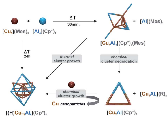
Scheme 2 Synthetic pathways to the new \text{Cu/Al} clusters [\text{Cu}_4\text{Al}_4](\text{Cp}^*)_5(\text{Mes}) ( 1 ), [\text{Cu}_2\text{Al}](\text{Cp}^*)_3 ( 2 ), and the inseparable mixture of [\text{HCu}_7\text{Al}_6](\text{Cp}^*)_6 ( 3 H ), [\text{Cu}_7\text{Al}_6](\text{Cp}^*)_6 ( 3 ), [\text{Cu}_8\text{Al}_6](\text{Cp}^*)_6 ( 4 ). \text{Cu} atoms are illustrated in orange, \text{Al} atoms in blue, respectively. For simplicity, only cluster cores are shown. All details of the experimental procedures and analytical characterization data are provided in the ESI.† Upon heating, cluster 1 can be transformed into a mixture of 3 , 3 H and 4 . This mixture can be selectively obtained by a sequence of cluster degradation and growth reactions with additives involving the trimetallic cluster intermediate 2 .
