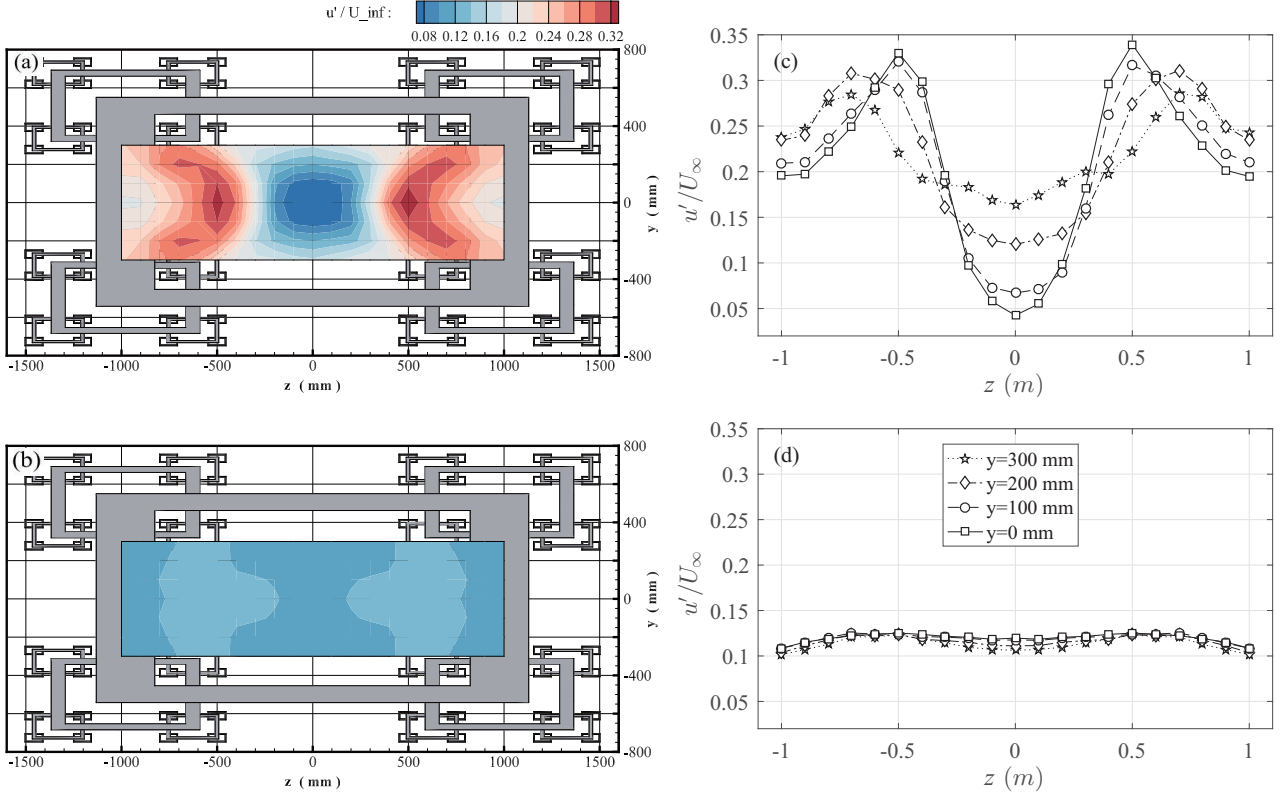
FIG. 15. Contours of u'/U_\infty at x/x_{peak} = 0.38 (a), and x/x_{peak} = 1.54 (b) at U_\infty = 10 m/s from the Honda experiments, assembled from (c) and (d), respectively.
