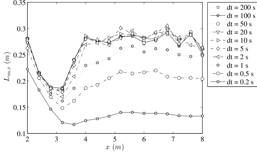
FIG. 28. Convergence of piecewise length in the calculation of L_u at U_\infty = 10 \text{ m s}^{-1} .
