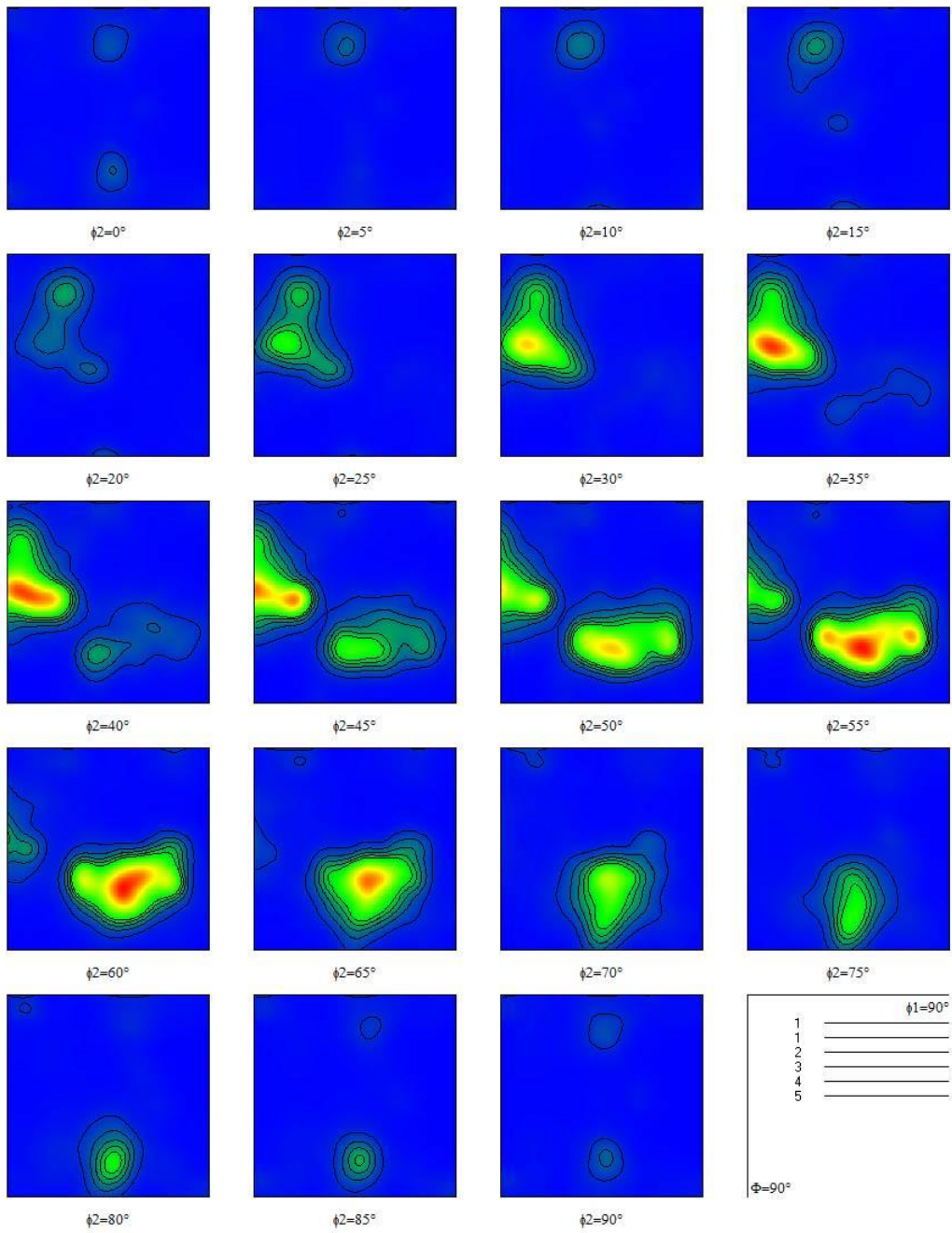
S.1 Orientation distribution function (ODF) of the HEA alloy
