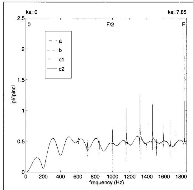
Figure 17. Far-field rigid backscattered normalized pressure spectrum.
