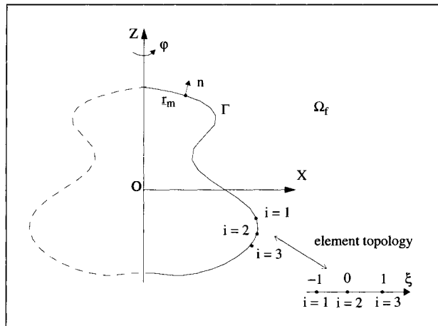
Figure 2. Axisymmetrical quadratic isoparametric element.
