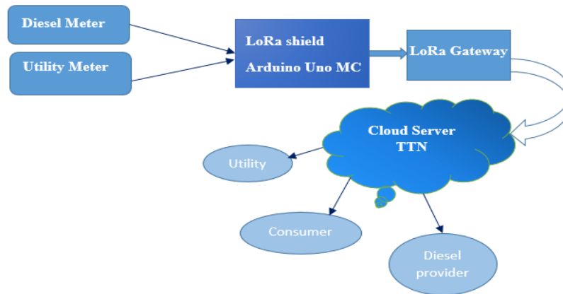
Fig. 6. LoRa module connected to energy Meters
