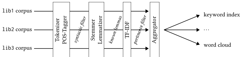
Figure 1: Keyword index generation pipeline
