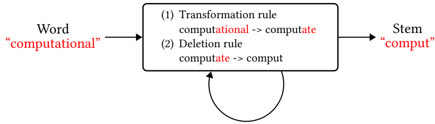
Figure 2: Ruled-based stemming
