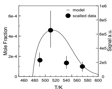
Figure 7. Comparison between experimental (symbols) and computed total mole fraction of KHPs (1000 ppm of DPE, \phi = 0.5 , 0.7 s, and 10 atm). The data are scaled to the computed maximum concentration. Experimental errors are estimated to be of the order of 40%.
