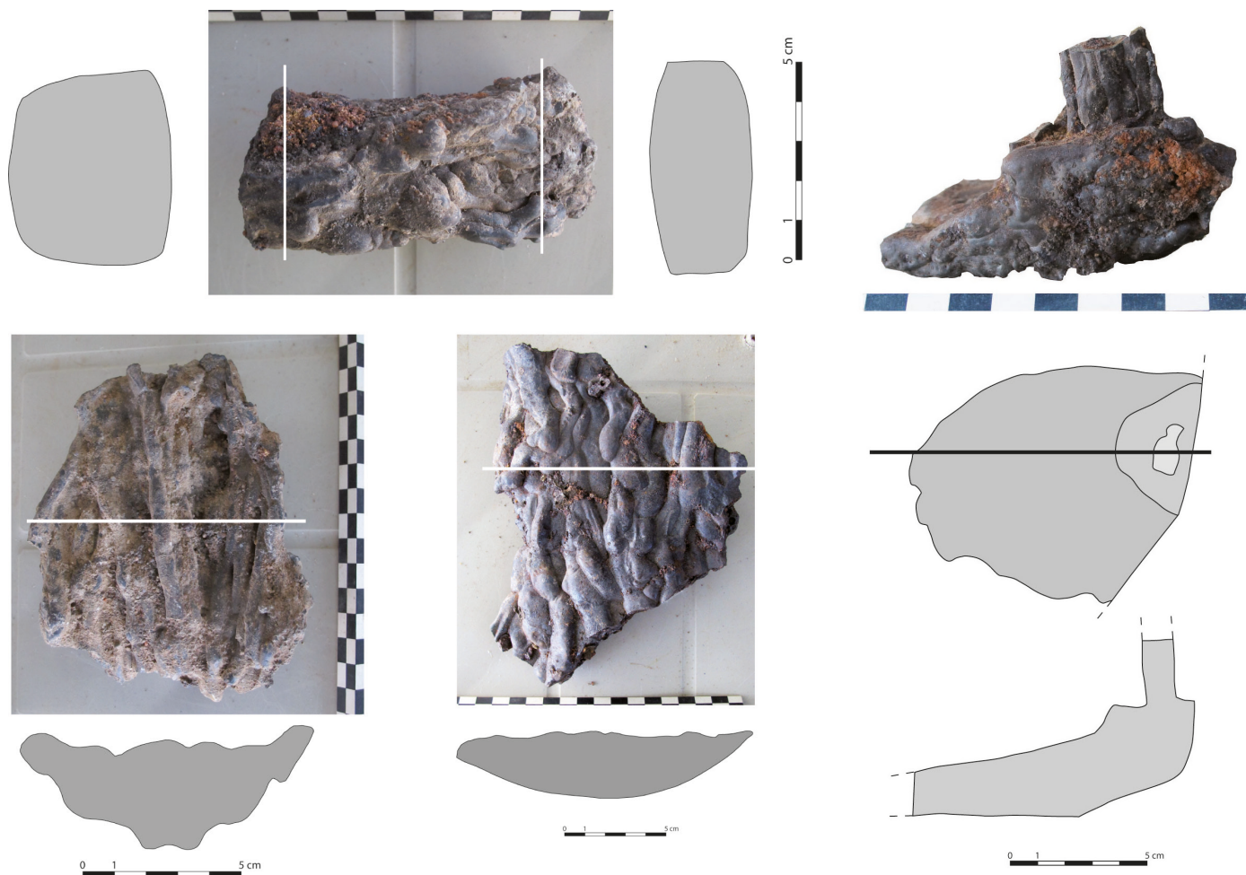
Figure 8. Cross section of the channels in which the slag flowed (MWS2002.28; MWS2006.10; MWS2002.24) (cl. N. Dieudonné-Glad, HeRMA, Université de Poitiers).
