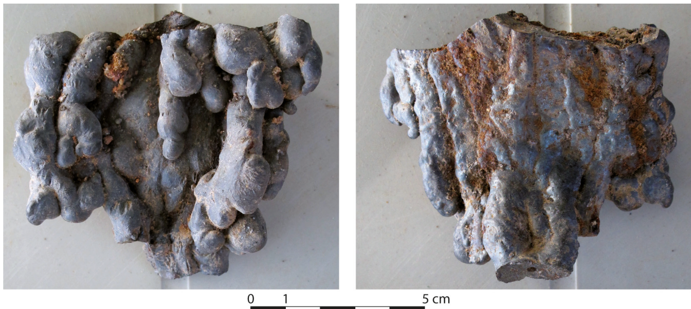
Figure 7. View of the upper and lower faces of a tapped slag (MWSS1C2.01) (cl. N. Dieudonné-Glad, HeRMA, Université de Poitiers).
