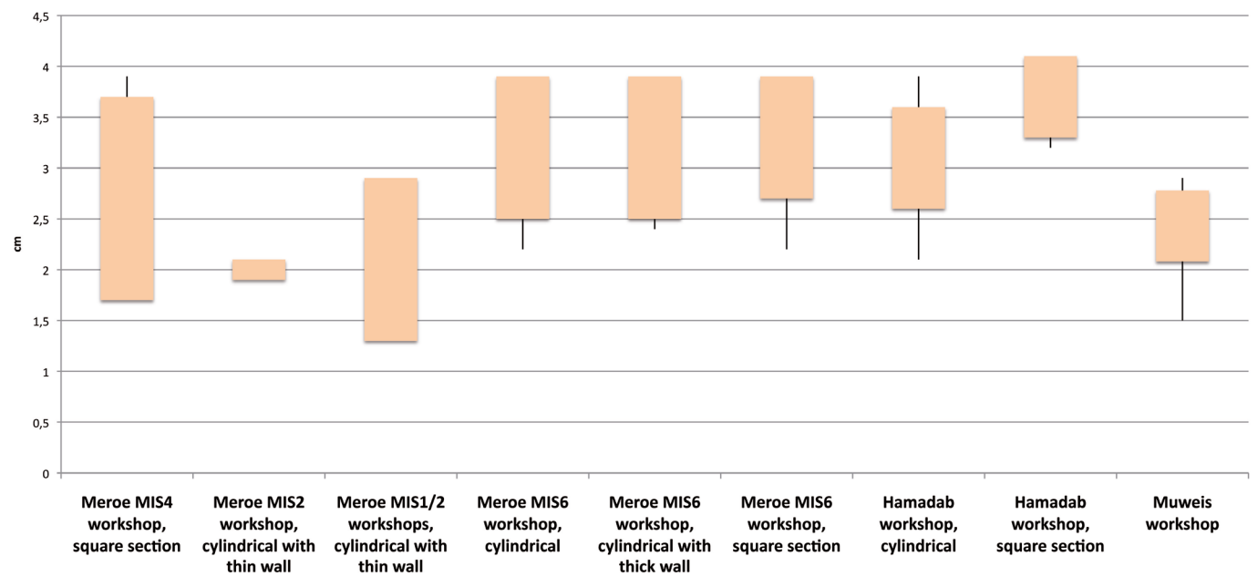
Figure 21. Diameter of the Muweis tuyere pipe compared to that of Meroe and Hamadab after Ting and Humphris 2017, table 3 (maximum, mean + standard deviation, mean-standard deviation, minimum).
