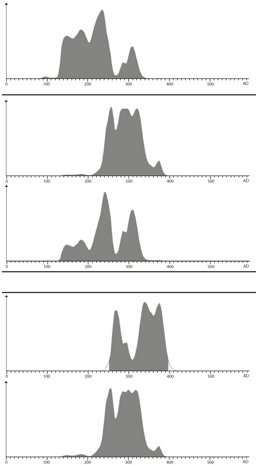
Figure 26. Calibrated radiocarbon dating (95% probability range) of stratigraphic layers of metallurgical material from mound. Top: dating of 1 charcoal from 2036 stratigraphic unit slag (UBA-30478, Age C14: 1803 +/- 29 years BP). Middle: dating of 2 charcoals from 2002 stratigraphic unit slag (ECHO1827, Age C14: 1750 +/- 25 years BP, ECHO1828, Age C14: 1785 +/- 25 years BP). Below: dating of 2 charcoals from 2036 stratigraphic unit slag (ECHO1829, Age C14: 1710 +/- 25 years BP, ECHO1830, Age C14: 1755 +/- 25 years BP).
