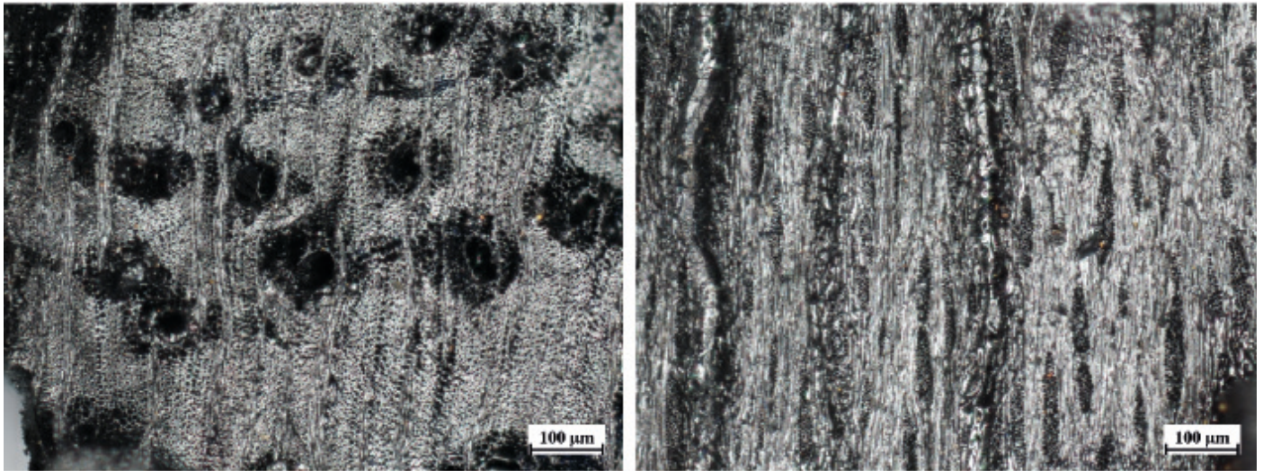
Figure 16. Microscope images of wood anatomical Acacia type nilotica , transverse section with vasicentric axial parenchyma (left) and longitudinal transversal section (right).
