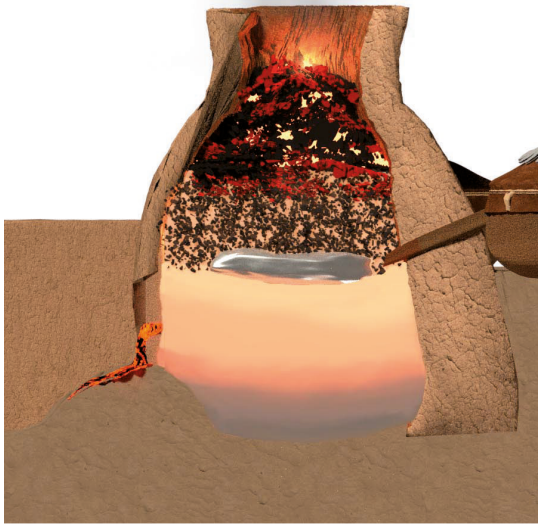
Figure 24. 3D model of a furnace interior during slag removal, based on the cross sections of the furnaces published by Shinnie (Shinnie and Kense 1982, fig.1, Shinnie and Anderson 2004, pl. Vb; 3D view: Etienne Chabrol, HeRMA, Université de Poitiers).
