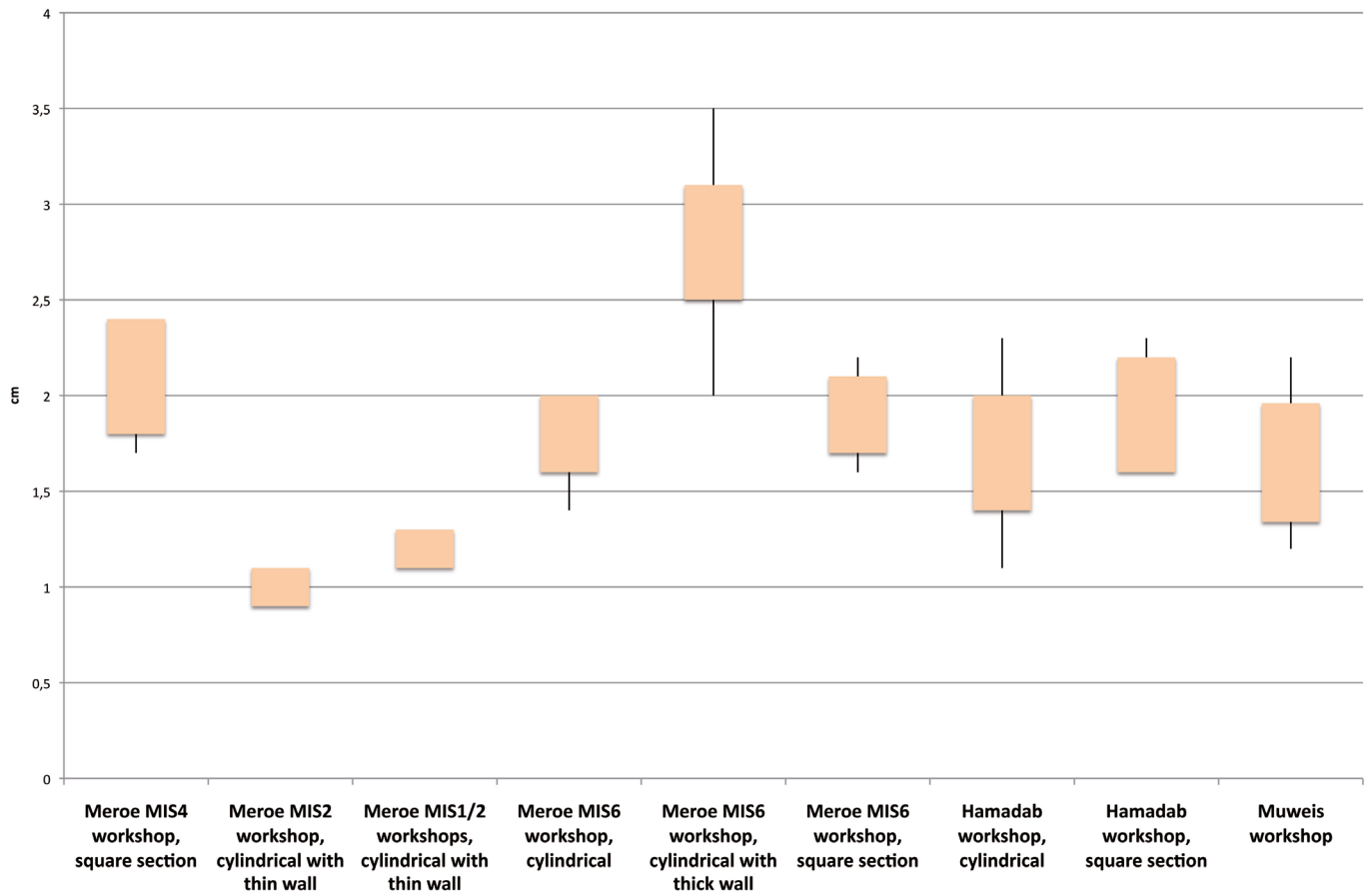
Figure 20. Thickness of the walls of the Muweis tuyeres compared to those of Meroe and Hamadab after Ting and Humphris 2017, table 3 (maximum, mean + standard deviation, mean - standard deviation, minimum).
