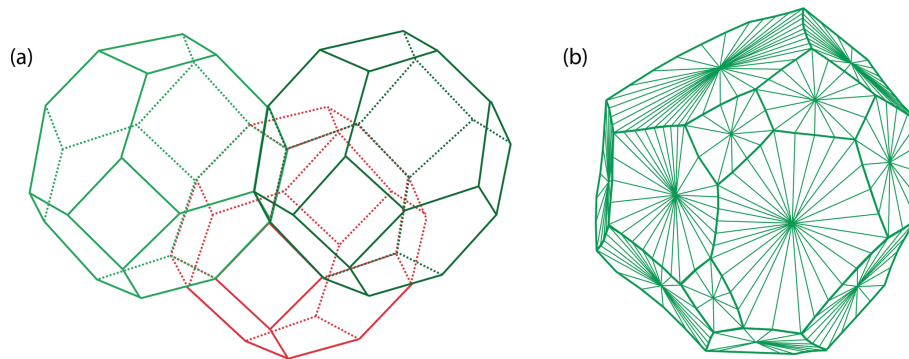
Figure 9. Grain shapes in polycrystalline materials: (a) the theoretical tetrakaidecahedral close-packed configuration with perfectly planar faces and (b) a simulated polyhedron grain with realistic curved faces (redrawn from Lazar et al., 2011).
