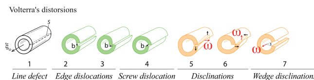
Figure 12. Volterra's distortions (Volterra, 1907). Sketches presenting the different types of deformation induced by (1) a line defect, (2–4) translation defects (dislocations) characterized by the Burgers vector \mathbf{b} , and (5–7) rotation defects (disclinations) characterized by the rotation vector \mathbf{f} (not shown; only the axis of rotation \omega is shown as a black arrow).
