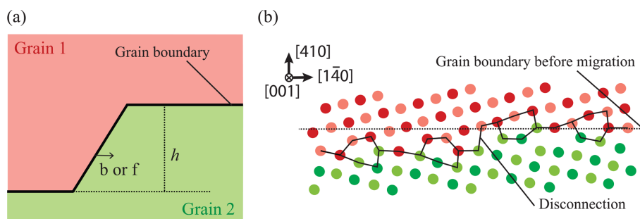
Figure 14. Disconnection along a grain boundary: “a defect inside a defect”. (a) A disconnection is characterized by a dislocation (with Burgers vector b ) and a step (height h ), or by the Frank vector f (e.g., generalized disclination; see Sun et al., 2018; Hirth et al., 2020). (b) An example of a disconnection along a Cu bi-crystal (grain boundary \Sigma 17(410) , redrawn from Combe et al., 2016). Dark and light green and red atoms do not have the same z coordinate.
