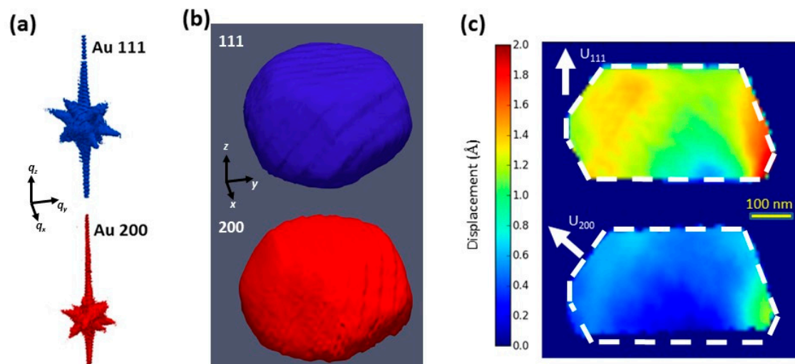
Figure 4. (a) 3D reciprocal space maps of the Au 111 and Au 200 Bragg peaks measured simultaneously using an Eiger 2 M and a MAXIPIX detector. (b) Isosurface of the Bragg electronic density reconstructed object from the Au 111 and 200 Bragg peaks. (c) Vertical cuts of the 3D displacement field component. The dotted white contours are guides for the eyes and delimit the shape of the crystal measured at the Au 111 Bragg reflection.
