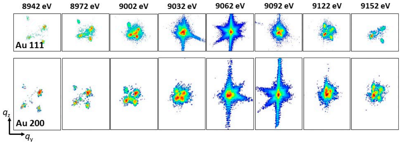
Figure 3. Sequences of 2D coherent diffraction patterns of the Au 111 and Au 200 Bragg peaks during a scan of the energy of the incident X-ray beam.
