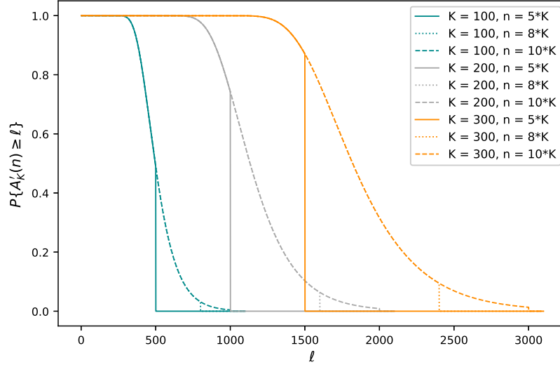
Figure 1: Using Theorem 4.6, we compute \mathbb{P}\{A'_K(n) \geq \ell\} for different values of K ( K = 100, 200 and 300 ) and at different collects n ( n = 5K, 8K and 10K ). The plain lines represent \mathbb{P}\{A'_{5K}(n) \geq \ell\} , the dotted lines represent \mathbb{P}\{A'_{8K}(n) \geq \ell\} and the dashed lines represent \mathbb{P}\{A'_{10K}(n) \geq \ell\} .
