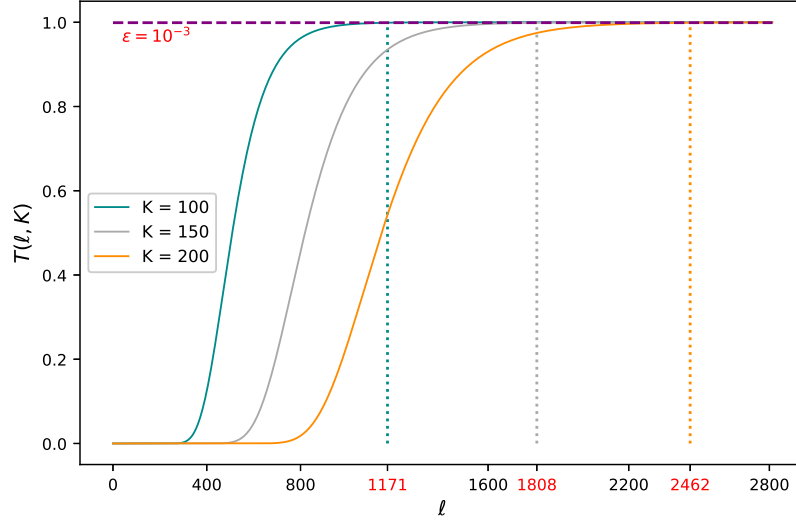
Figure 2: Illustration of the stationary maximal amount of uncollected data over the K end-devices. For K = 100, 150 and 200 and for each \ell = K, \dots, 2,800 , we compute T(\ell, K) and thresholds \ell(K, \varepsilon) for \varepsilon = 10^{-3} (i.e., \ell(100K, \varepsilon) = 1171 , \ell(150K, \varepsilon) = 1808 , and \ell(200K, \varepsilon) = 2462 ). The purple line represents 1 - \varepsilon = 0.999 .
