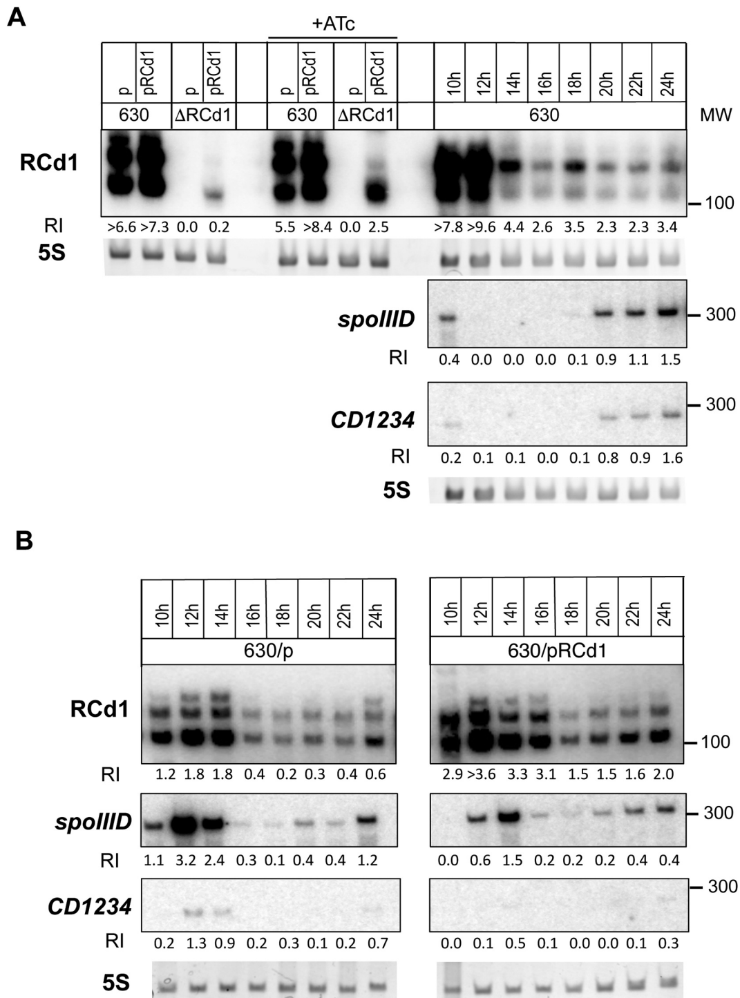
Figure 6. The expression profile of RCd1 and selected potential targets during sporulation. (A) RNA samples were extracted from 630Δ erm strain (630), 630Δ erm strain carrying an empty vector (630/p) or overexpressing RCd1 from plasmid (630/pRCd1) grown in TY medium supplemented on not with 250 ng/ml ATc (+ATc) or in SM medium for 10 h, 12 h, 14 h, 16 h, 18 h, 20 h, 22 h, 24 h as indicated. The strain deleted for RCd1 (ΔRCd1) was used as a control for specific RCd1 detection. 5S RNA at the bottom serves as loading control. As indicated at the left, the blots were hybridized either with RCd1, spoIIID or CD1234 -specific probes. The same 5S control panel is shown when reprobing of the same membrane was performed. Relative intensity of the bands 'RI' normalized to 5S estimated with ImageJ software is indicated underneath each lane, '>' indicates the saturation of the signal. MW, the size of RNA molecular weight standards in nucleotides. (B) Effect of RCd1 overexpression on spoIIID and CD1234 genes during sporulation was monitored in SM medium during sporulation for 10 h, 12 h, 14 h, 16 h, 18 h, 20 h, 22 h, 24 h as indicated.
