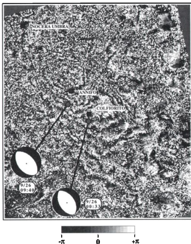
Figure 1. SAR differential interferogram of the Colfiorito area showing the total surface displacement occurred between September 7 and October 12, 1997. Each fringe represents a full phase cycle ( +\pi - \pi ) caused by a displacement increment of -28 mm in the slant range; the direction of the increment is from the outermost fringe inward. Also shown are the epicentral location of the two September, 26, shocks and the CMT focal mechanisms (after Ekström et al. , [1998]). To better retain the details of the fringe pattern, the image is not geocoded (SAR geometry). The small residual fringes visible towards the extreme right of the image are presumably related to propagation delays due to tropospheric turbulence.
