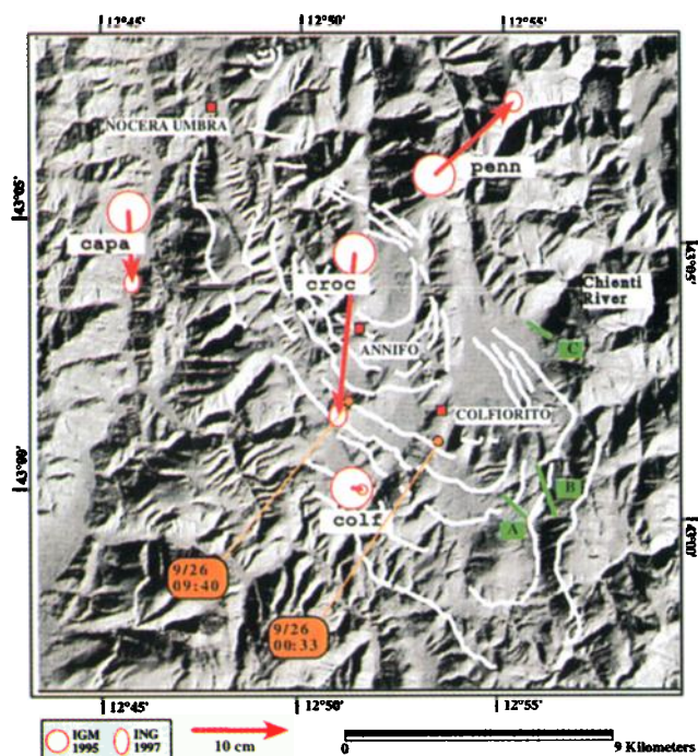
Figure 2. Geocoded displacement contours retrieved from the interferogram in figure 1. Each contour line represents a displacement increment of -28 mm in the slant range. GPS stations (in lowercase), planar displacement vectors (red arrows), and 95% confidence error ellipses for the 1995 and 1997 epochs (see Table 1), are shown. A and B are the traces of the bedrock fault plane reactivations (after Basli et al. , [1998]). C is the location of the scarp damming the outlet of the Colfiorito basin.
