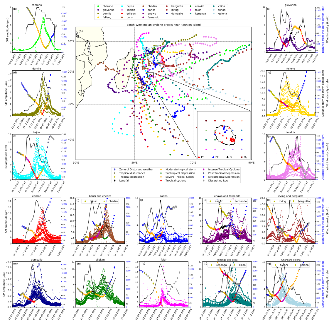
Figure 8. SM signatures of cyclones at La Réunion seismic stations. (a) Tracks of the tropical cyclones that passed close to Réunion Island between 2011 and 2019 (distance station-to-storm center <500 km). The inset map shows the seismic stations onland (in red from the OVPF and in blue from the ZF temporary network) and the offshore node locations at which the modeled H_S are extracted. (b–q) Each subplot shows the RMS amplitude of the SM (colored dots, left axis) for each selected cyclone, together with the distance between the storm center and the seismic station plotted as colored diamonds (on the right axis, blue scale) and the cyclone intensity plotted as continuous black lines (right axis, black scale). For each cyclone, the RMS amplitude at the various stations is plotted with the same color code as the track on the map Figure 8a. All seismic stations have the same color.
