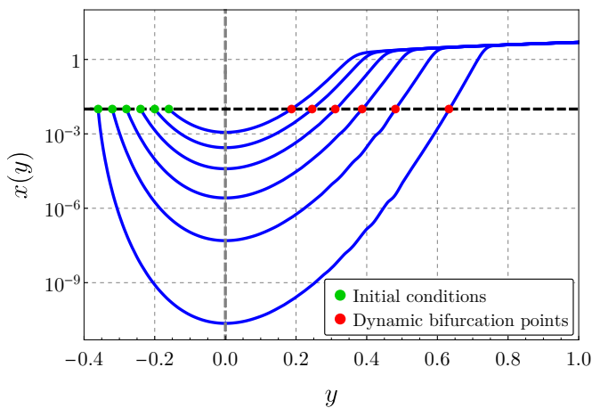
Figure 3. Numerical simulations of the deterministic differential equation associated to Eq. (29) using a logarithm scale for the vertical axis. The set of parameters (45) is used with, in addition, x(y_0) = 0.01 (the latter is depicted by a horizontal dashed line) and y_0 = -0.36, -0.32, \dots, -0.16 . The static bifurcation point \hat{y}^{\text{st}} = 0 is depicted by a vertical gray dashed line. The dynamic bifurcation point \hat{y}_{\text{det}}^{\text{dyn}} is defined for a given initial condition by the value of y for which |x(y)| = |x(y_0)| , which corresponds graphically to the intersection between the blue curves and the horizontal dashed line. The green and red points are used respectively to highlight the considered initial conditions and the corresponding dynamic bifurcation points predicted by Eq. (42).
