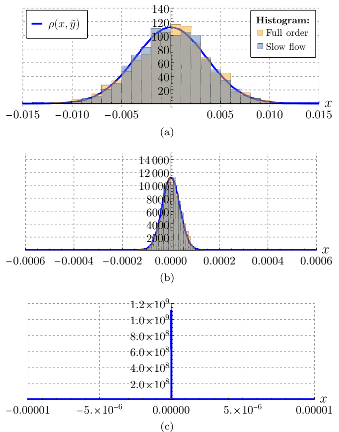
Figure 11. Comparison between theoretical PDF \rho(x, y) given by Eq. (63) and two histograms: one built from the full order system (11) and the other from the stochastic slow dynamics (29). In both cases, 2000 realizations of the system are computed and we take, for each realization, the value of the considered random variable ( x_y or p_t ) for a given value of y denoted \tilde{y} (chosen arbitrary to be \tilde{y} = 0.15 ). The comparison is performed for three values of the noise level: (a) \sigma = 10^{-4} , (b) \sigma = 10^{-6} and (c) \sigma = 10^{-11} . Moreover y_0 = -0.34 , x_{y_0} = 0.01 and \epsilon = 0.002 .
