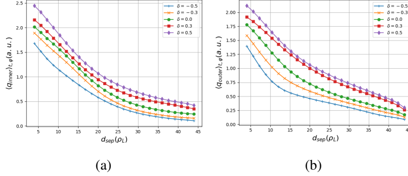
Figure 3: a) inner and b) outer targets radial profiles for different triangularities values ( -0.5 + , -0.3 \times , 0.0 \bullet , +0.3 \blacksquare , +0.5 \blacklozenge ). The profiles are remapped to LFS midplane of circular simulation for relevant comparison. On both inner and outer targets, the peak value of the heat flux q_0 and the SOL power fall-off length remapped at LFS MP \lambda_q are decreased from positive to negative triangularity values. The detailed values are resumed in table 3. The conservation of the energy is assured by the increase of the limiter surface from positive to negative triangularity simulations.
