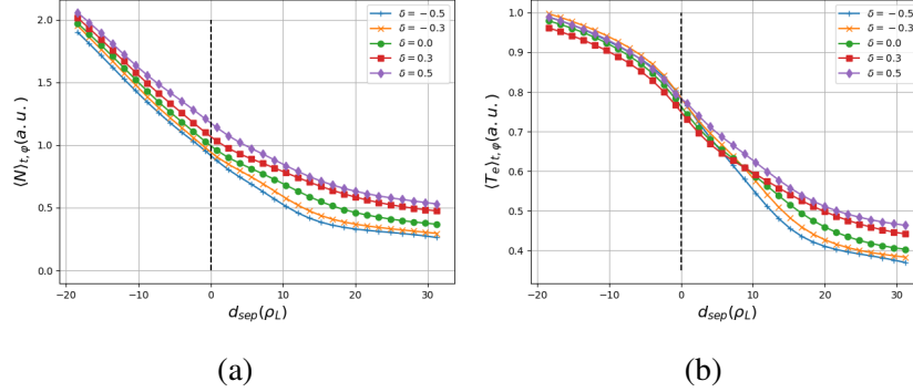
Figure 2: Low Field Side Midplane (LFS MP) profiles of average on time and toroidal position of a) Density and b) Electron Temperature for different negative triangularities values ( -0.5 \times , -0.3 \times , 0.0 \bullet , +0.3 \blacksquare , +0.5 \blacklozenge ). The dashed line represents the position of the separatrix which defines the frontier between the edge closed field lines region (CFR) on its left and the scrape-off layer (SOL) open field lines region on its right. For both density and electron temperature, the impact of triangularity is weaker in the edge closed field lines region compared to the SOL. From positive to negative triangularity simulations, averaged density is reduced and steepened in both the edge closed field lines region and the SOL. Average electron temperature radial profiles are also steepened in the SOL from \delta > 0 to \delta < 0 but no clear trend is visible in the edge closed field lines region. The steepening in the SOL of both average density and electron temperature gradients are measured with an exponential fit and the values of the characteristic decay lengths L_N and L_{T_e} are resumed in table 2.
