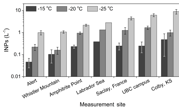
Figure 2. Mean INP number concentrations at droplet freezing temperatures of -15\text{ }^{\circ}\text{C} (dark gray), -20\text{ }^{\circ}\text{C} (intermediate gray), and -25\text{ }^{\circ}\text{C} (light gray). Uncertainty is given as the standard error of the mean, assuming a normal distribution. As only one sample was available from the Labrador Sea, no uncertainty is reported.
